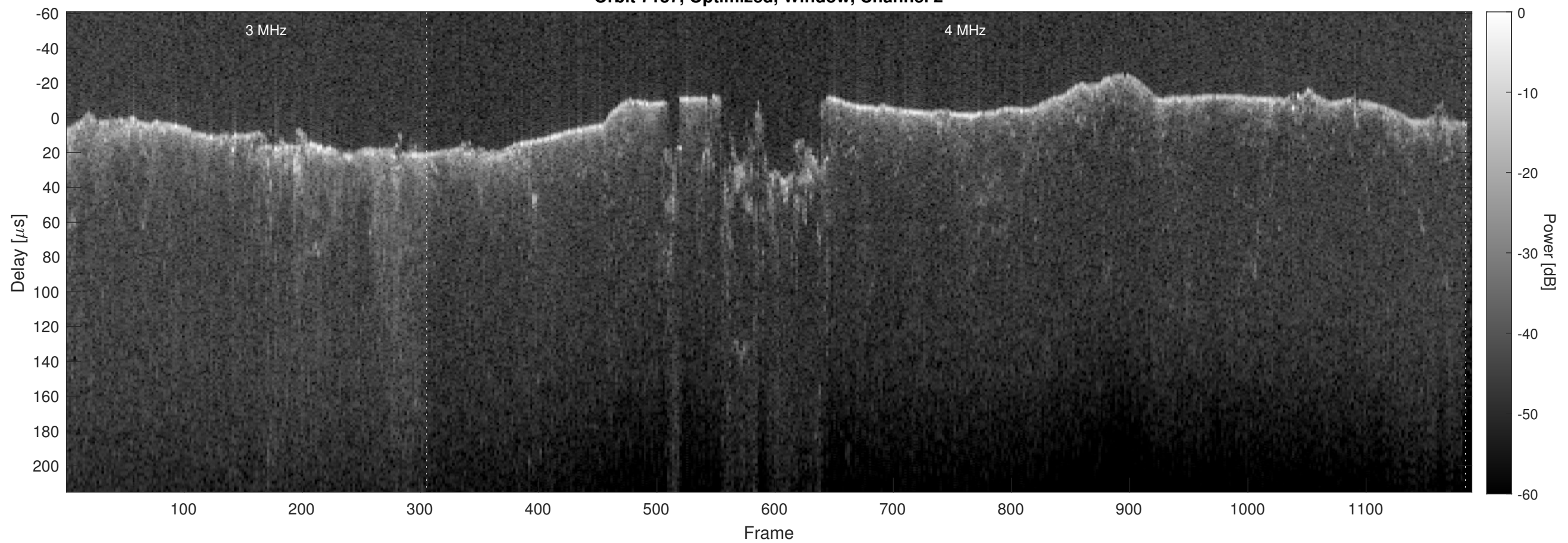
Orbit 7137, Optimized, Window, Channel 2
