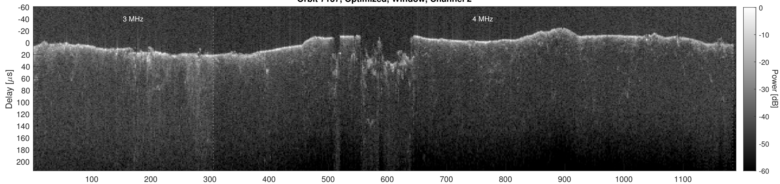
Orbit 7137, Cluttergram
