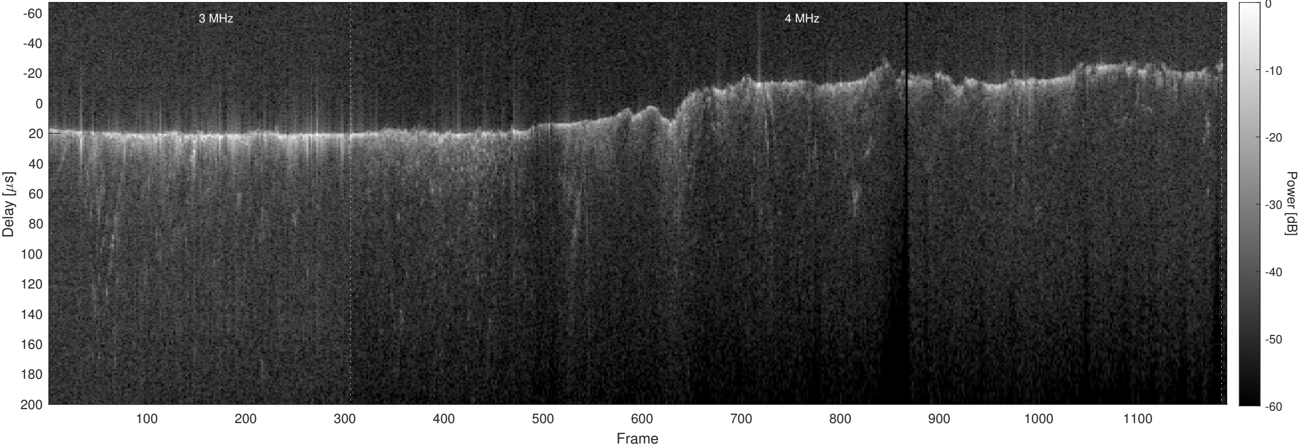
Orbit 7138, Optimized, No Window, Channel 2
