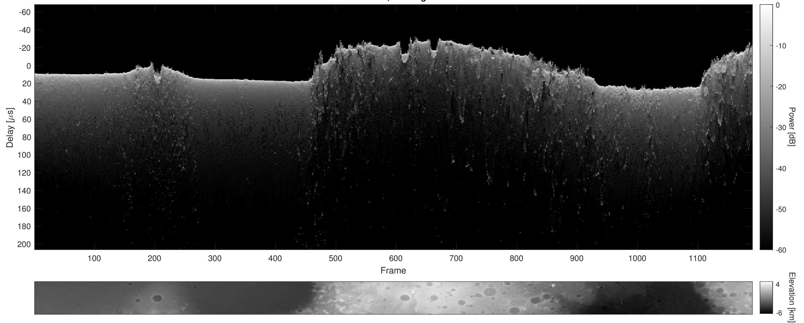
Orbit 7139, Cluttergram
