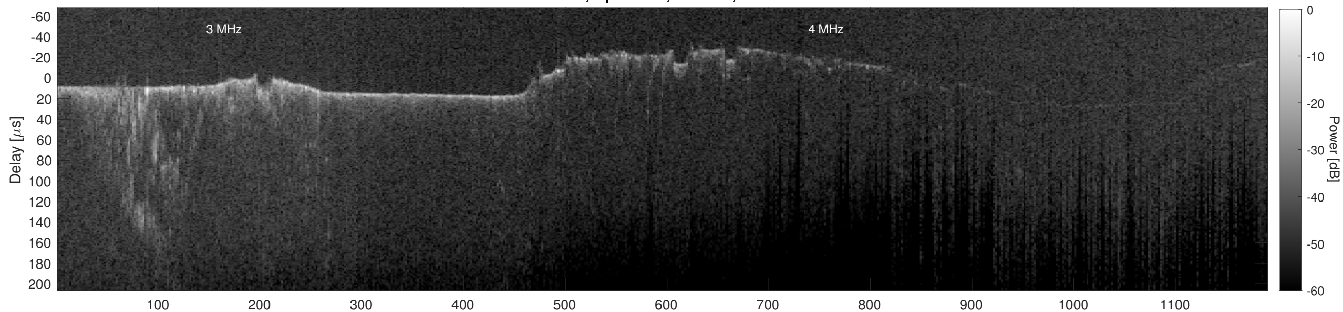
Orbit 7139, Cluttergram
