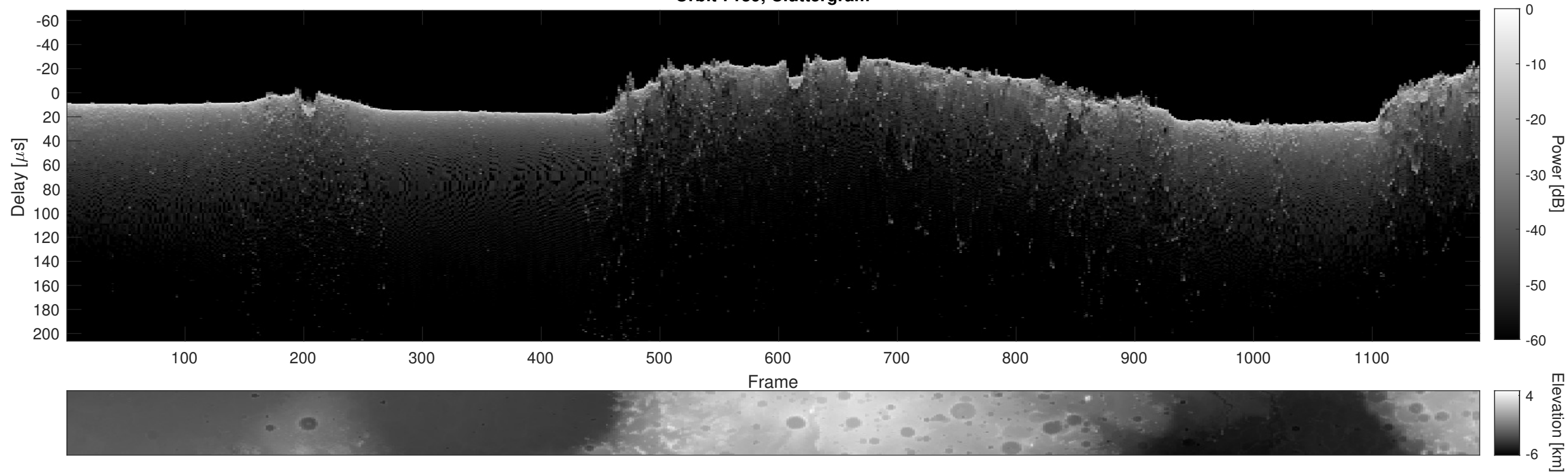
Orbit 7139, Cluttergram
