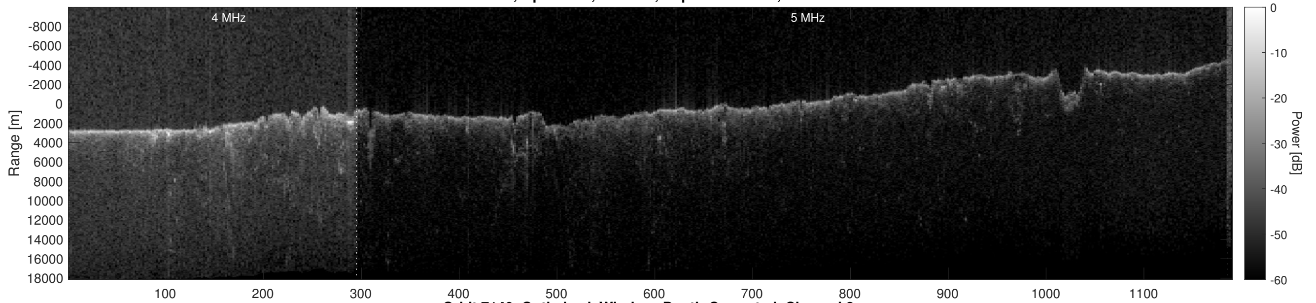
Orbit 7140, Optimized, Window, Depth-Corrected, Channel 2
