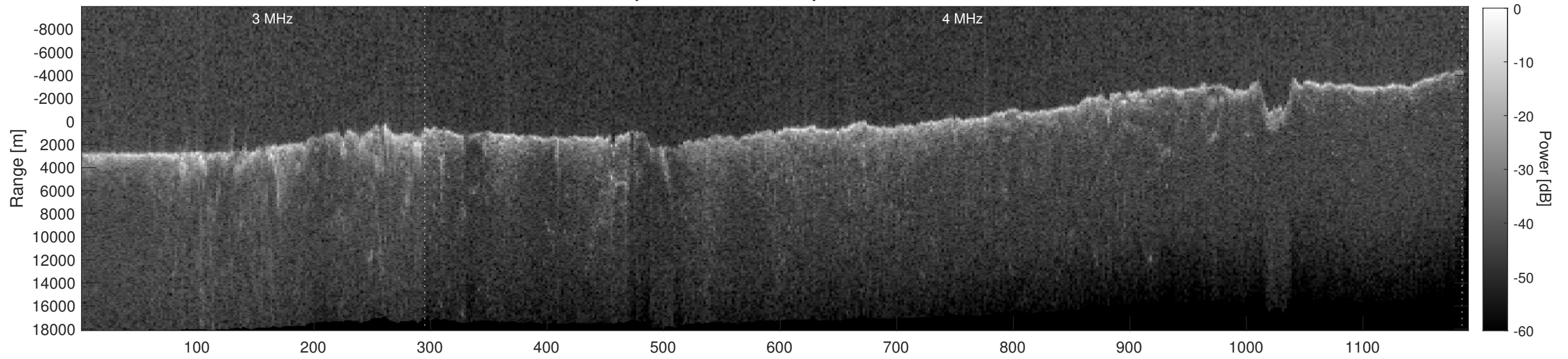
Orbit 7140, Depth-Corrected Cluttergram
