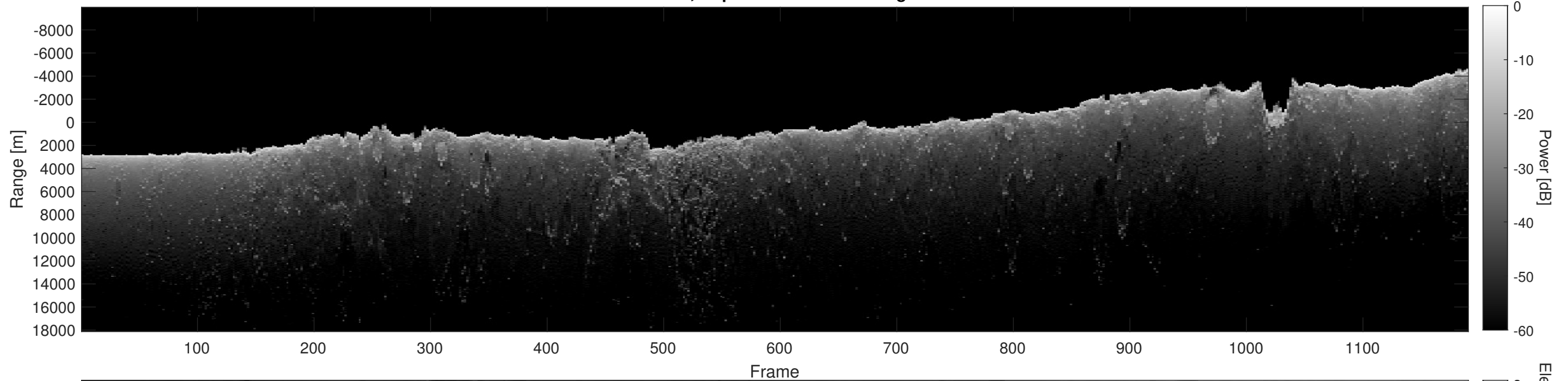
Orbit 7140, Depth-Corrected Cluttergram
