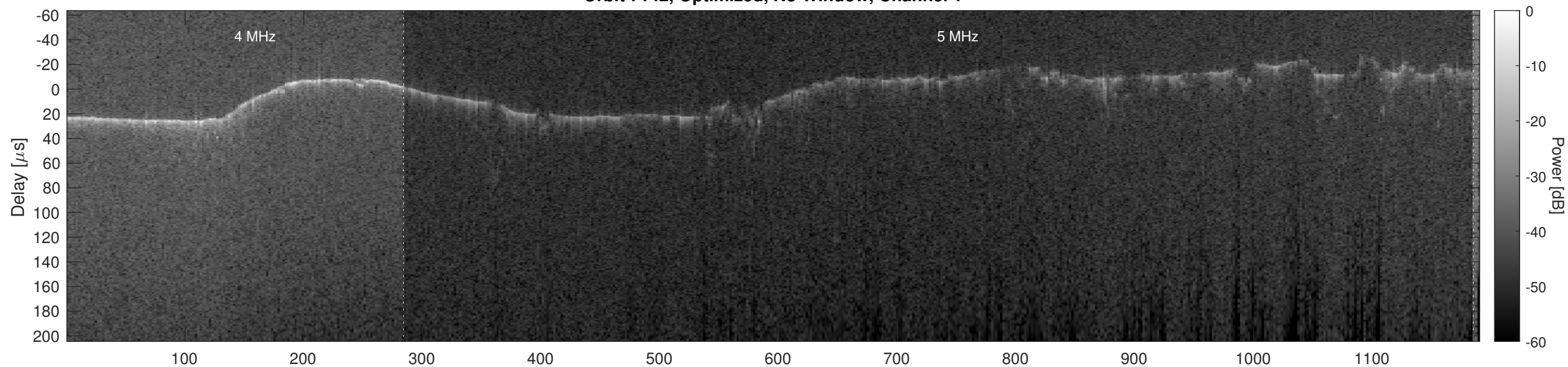
Orbit 7142, Optimized, No Window, Channel 2
