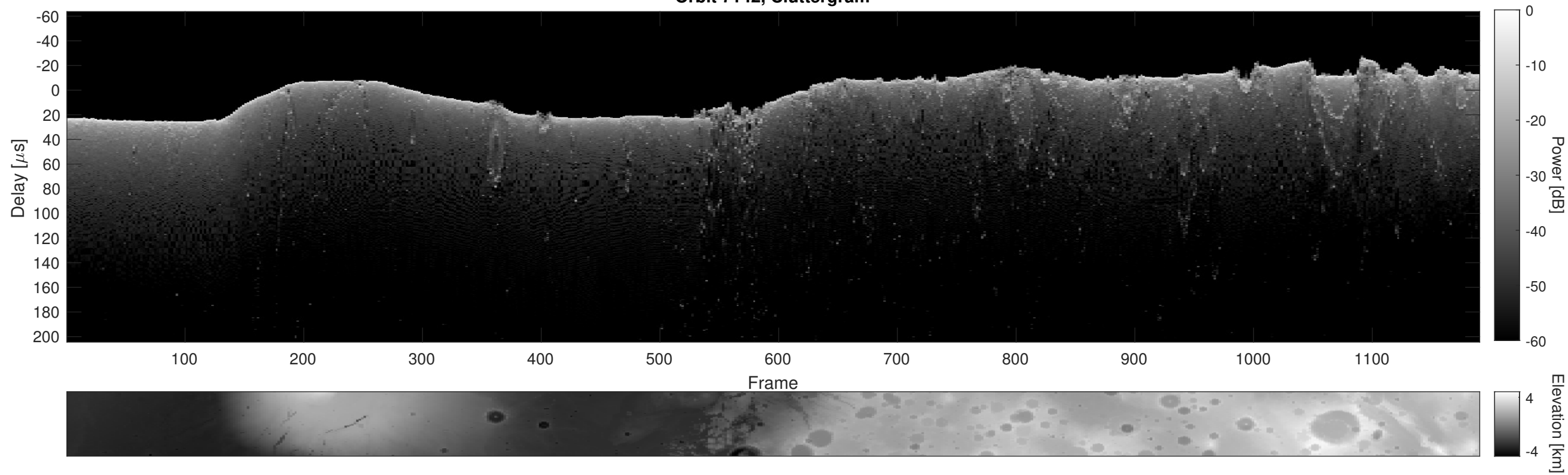
Orbit 7142, Cluttergram
