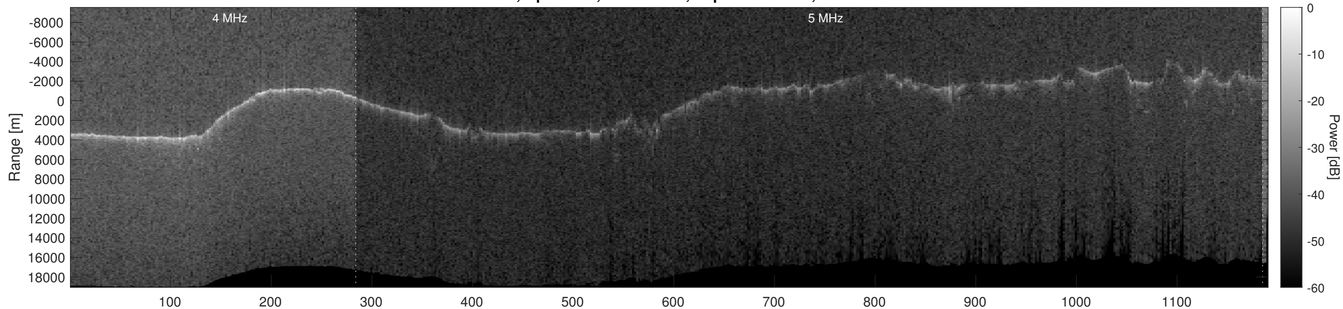
Orbit 7142, Optimized, No Window, Depth-Corrected, Channel 2
