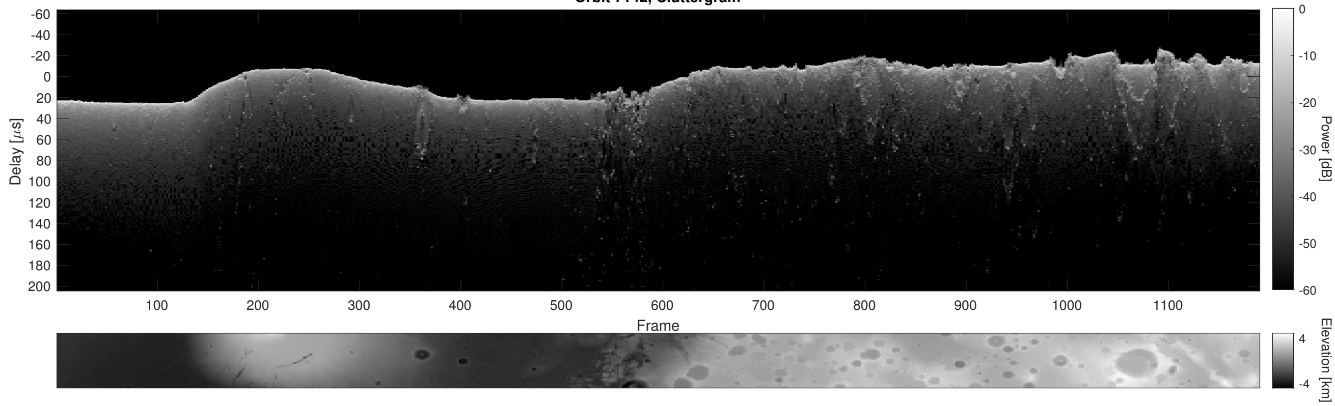
Orbit 7142, Cluttergram
