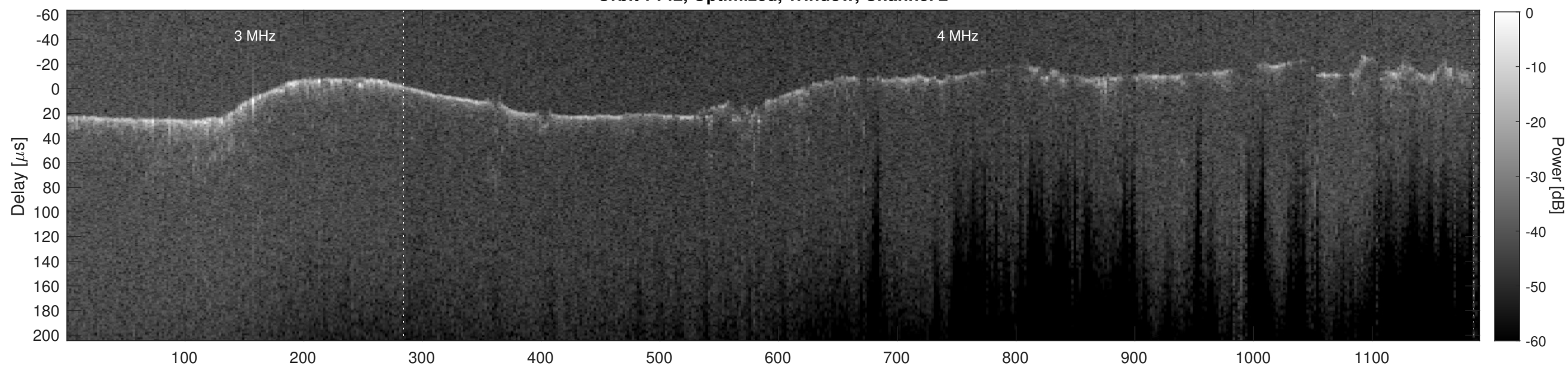
Orbit 7142, Cluttergram
