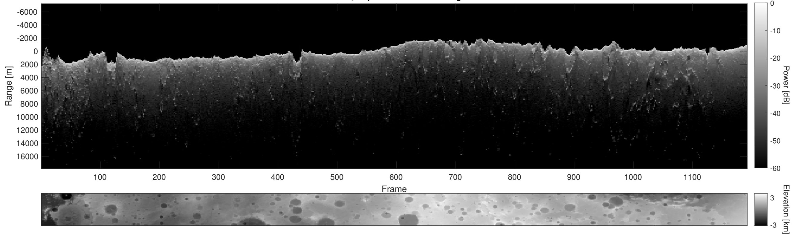
Orbit 7143, Depth-Corrected Cluttergram
