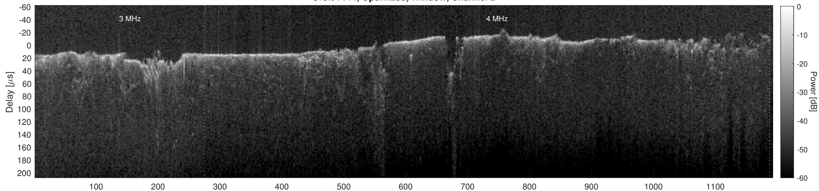
Orbit 7144, Cluttergram
