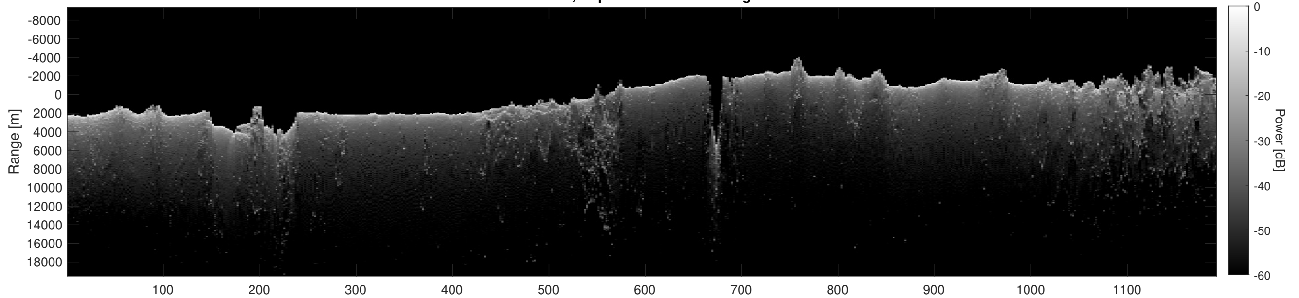
Orbit 7144, Depth-Corrected Cluttergram
