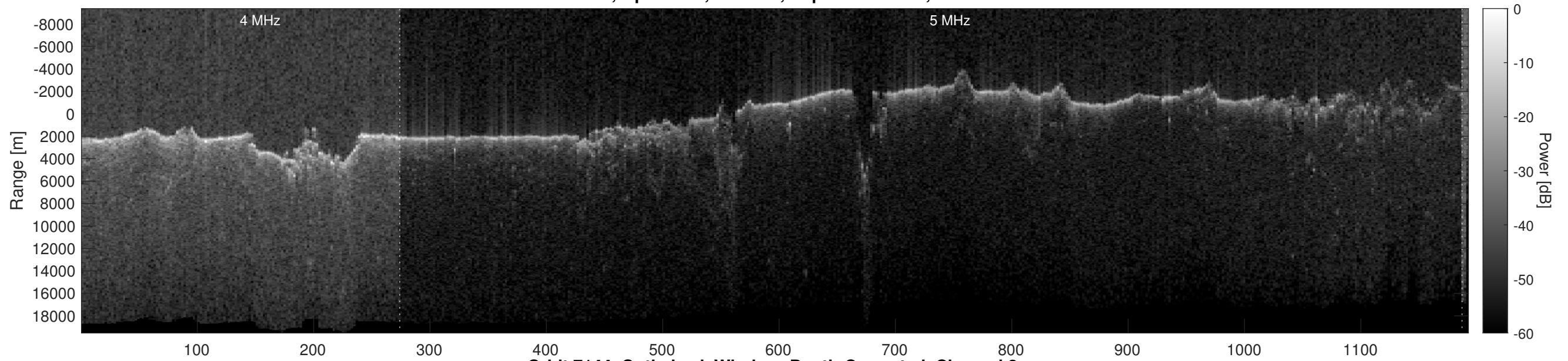
Orbit 7144, Optimized, Window, Depth-Corrected, Channel 2
