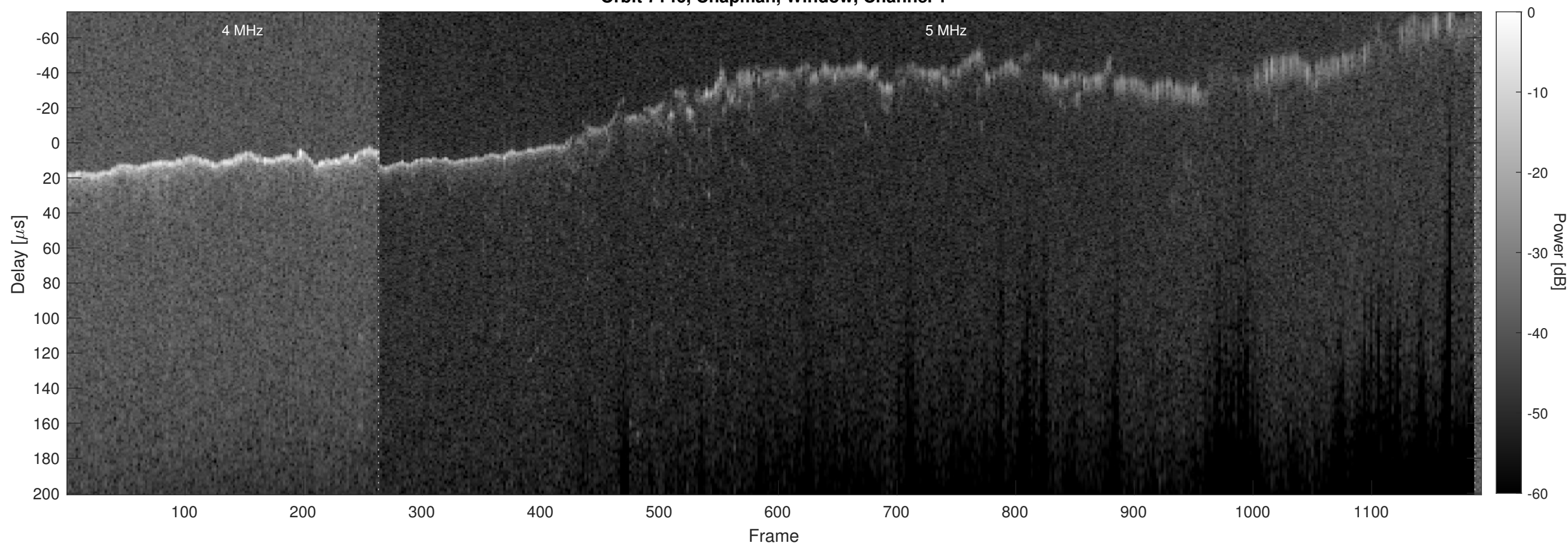
Orbit 7146, Chapman, Window, Channel 2
