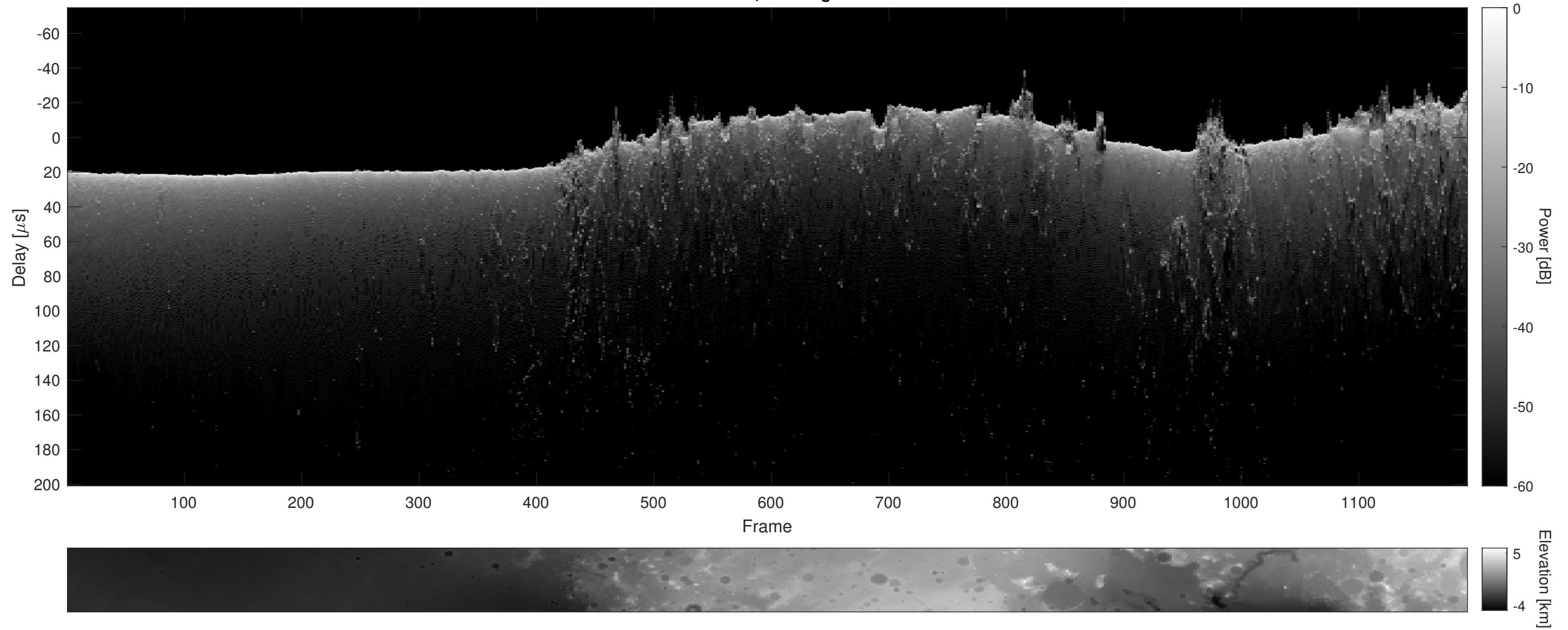
Orbit 7146, Cluttergram
