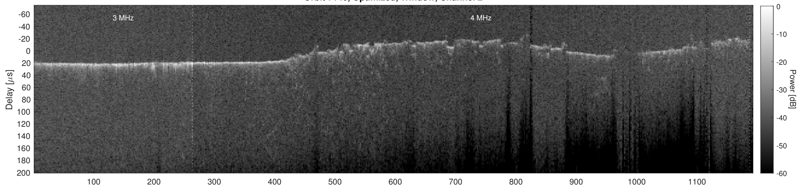
Orbit 7146, Cluttergram
