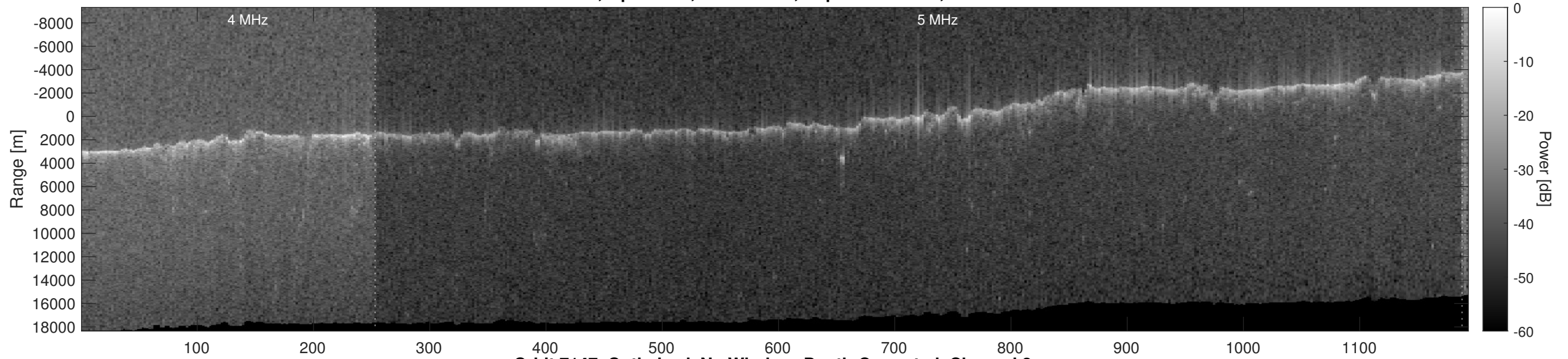
Orbit 7147, Optimized, No Window, Depth-Corrected, Channel 2
