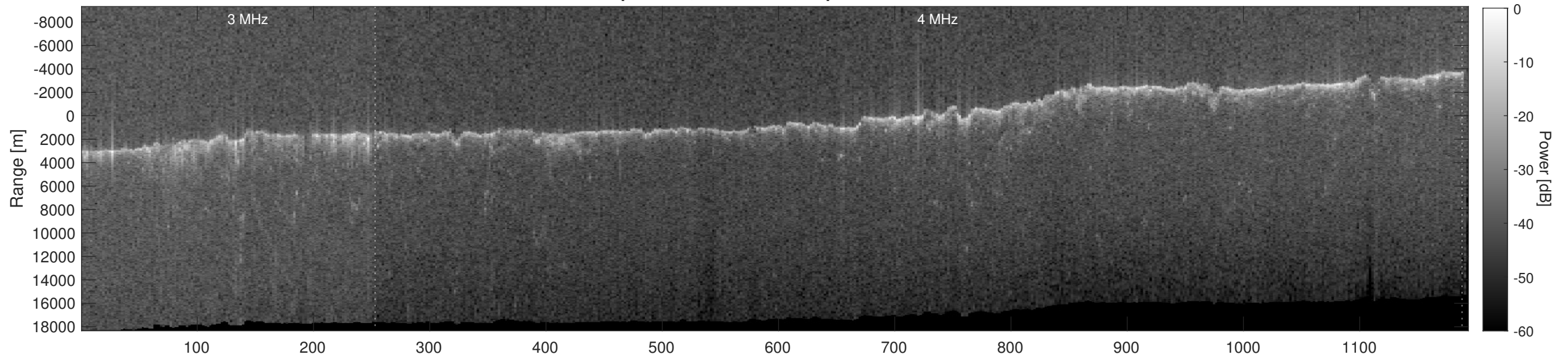
Orbit 7147, Depth-Corrected Cluttergram
