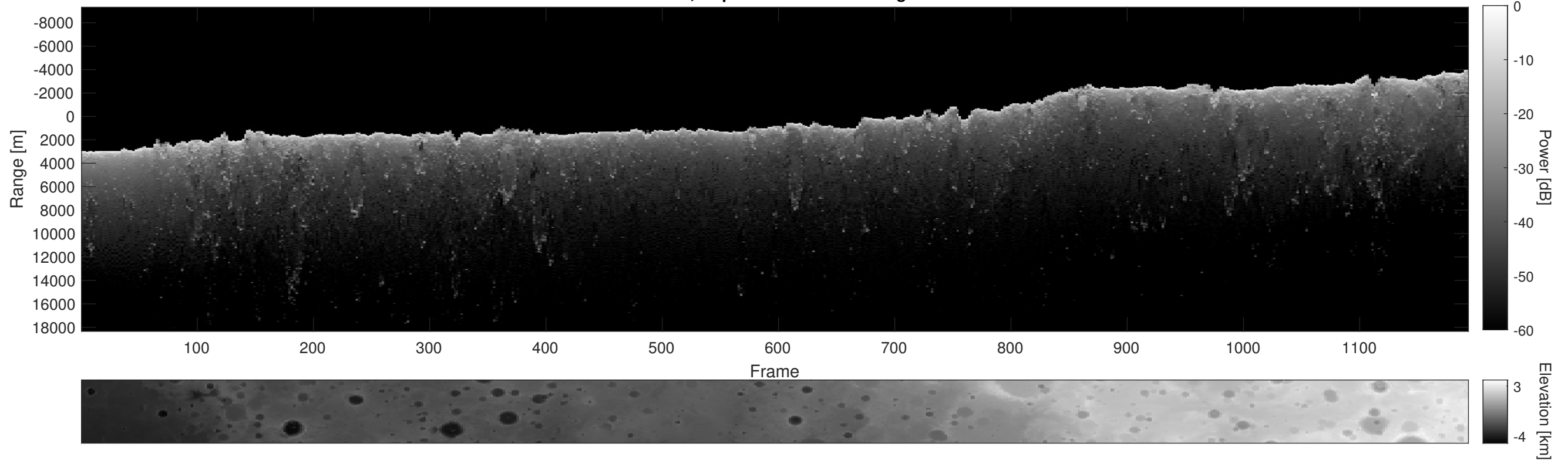
Orbit 7147, Depth-Corrected Cluttergram
