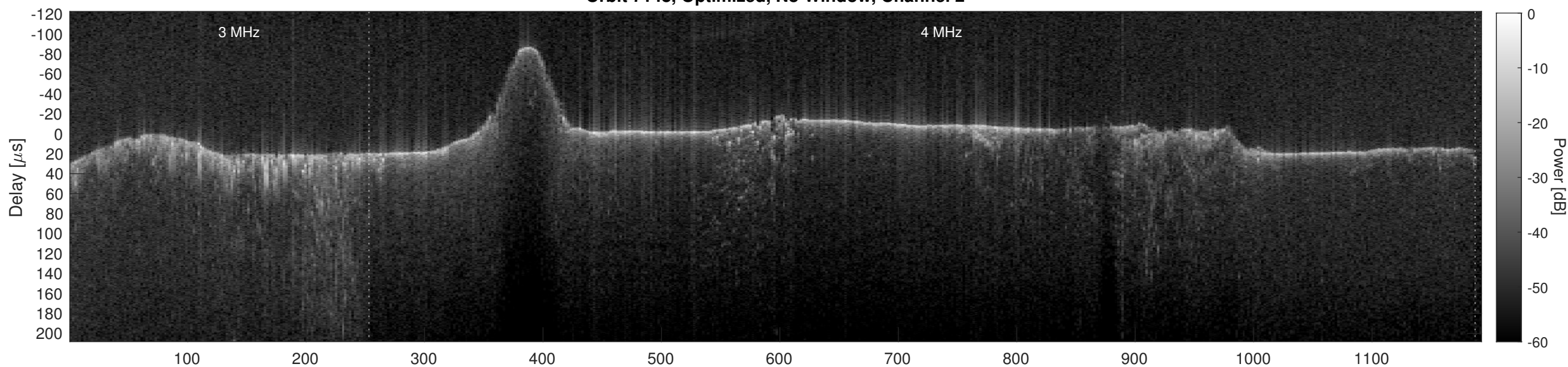
Orbit 7148, Cluttergram
