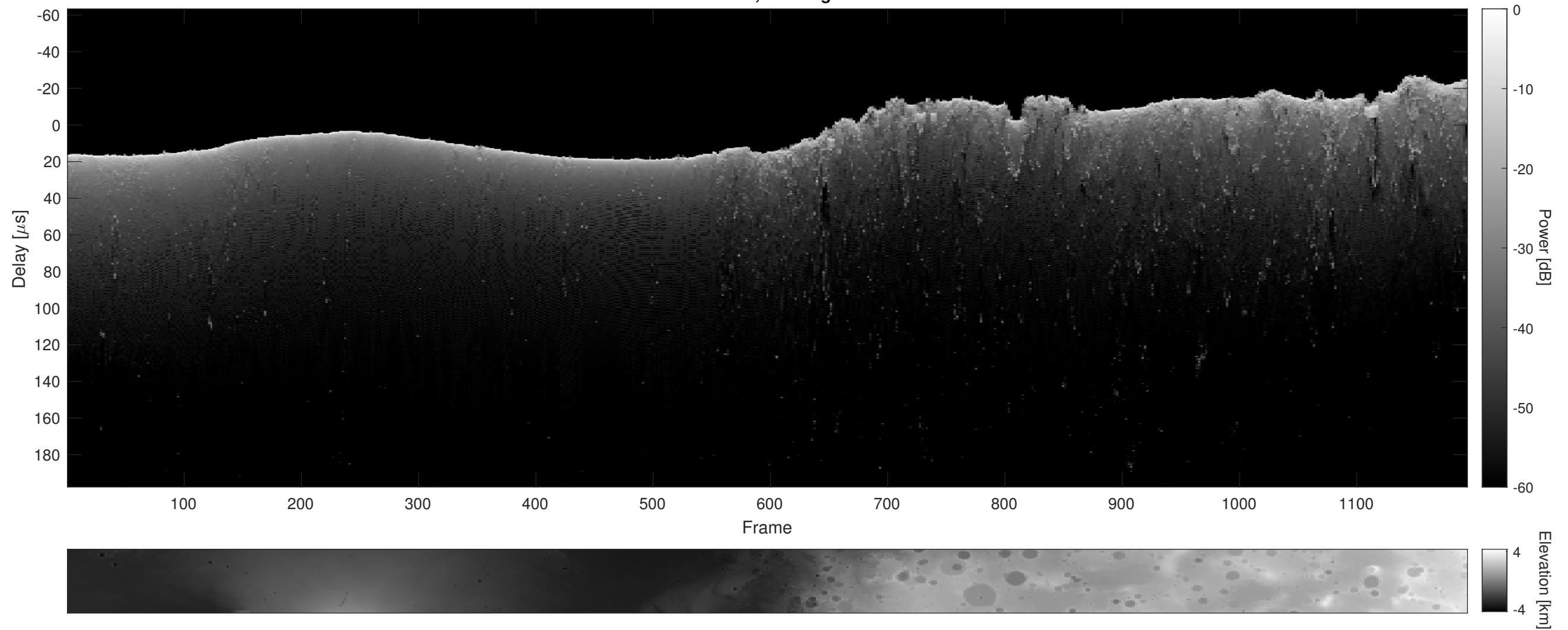
Orbit 7149, Cluttergram
