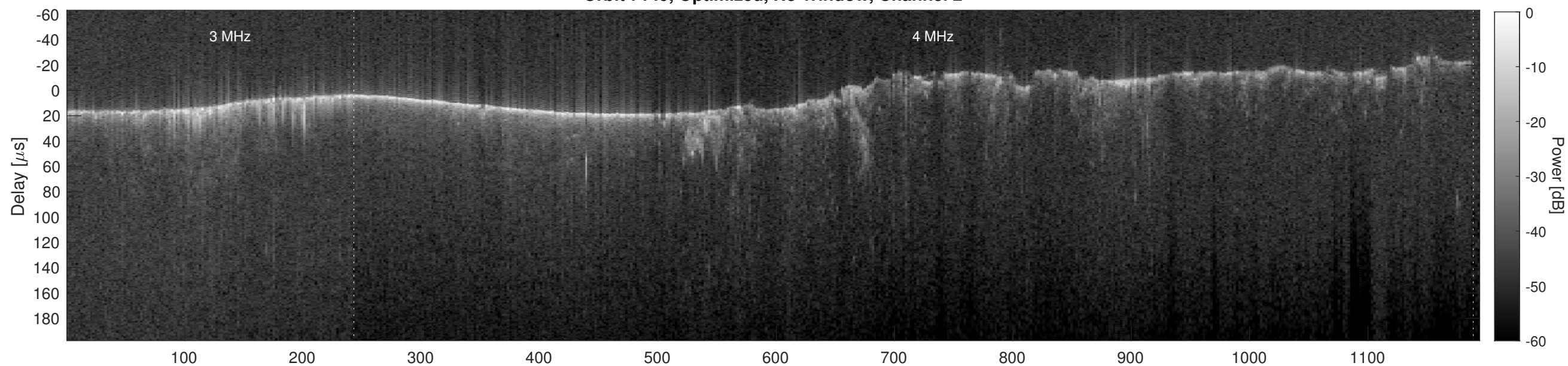
Orbit 7149, Cluttergram
