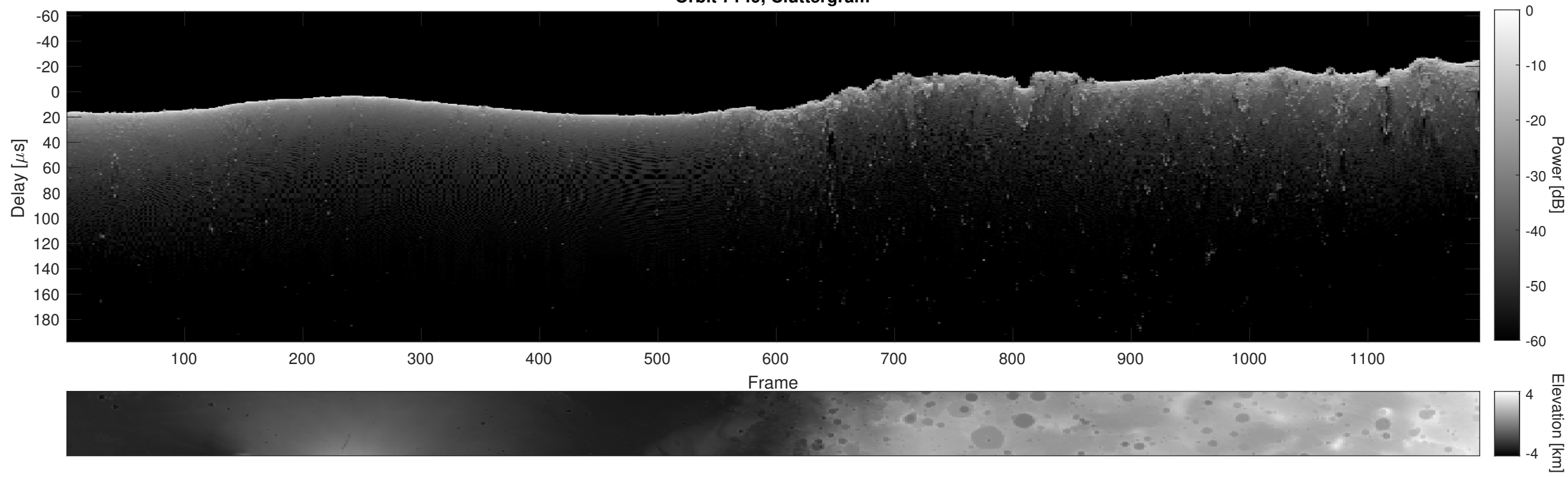
Orbit 7149, Cluttergram
