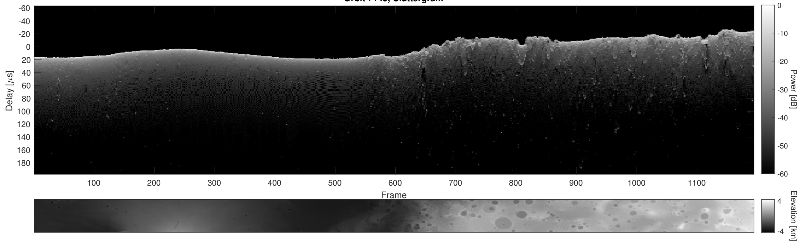
Orbit 7149, Cluttergram
