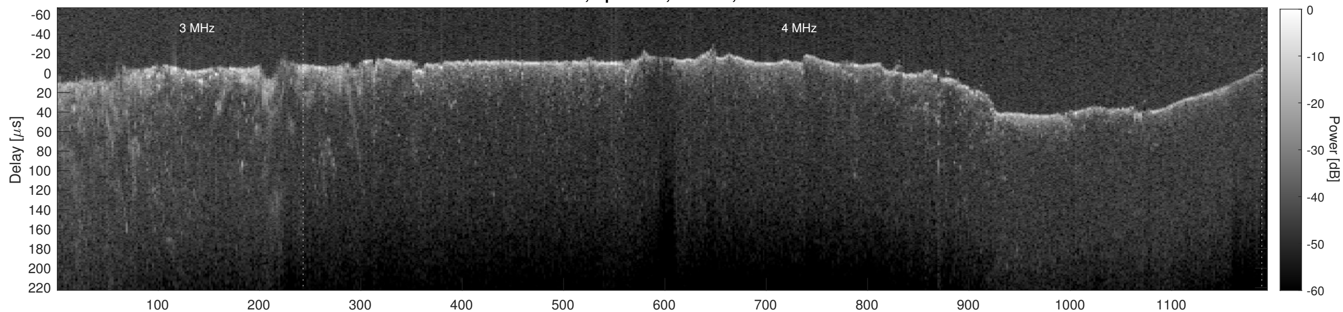
Orbit 7150, Cluttergram
