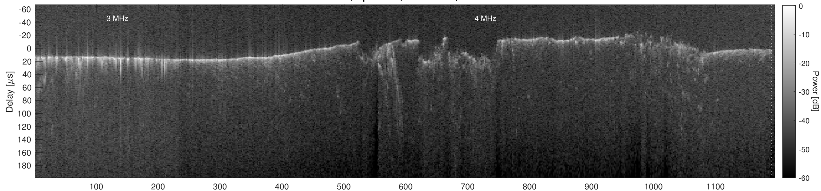
Orbit 7151, Cluttergram
