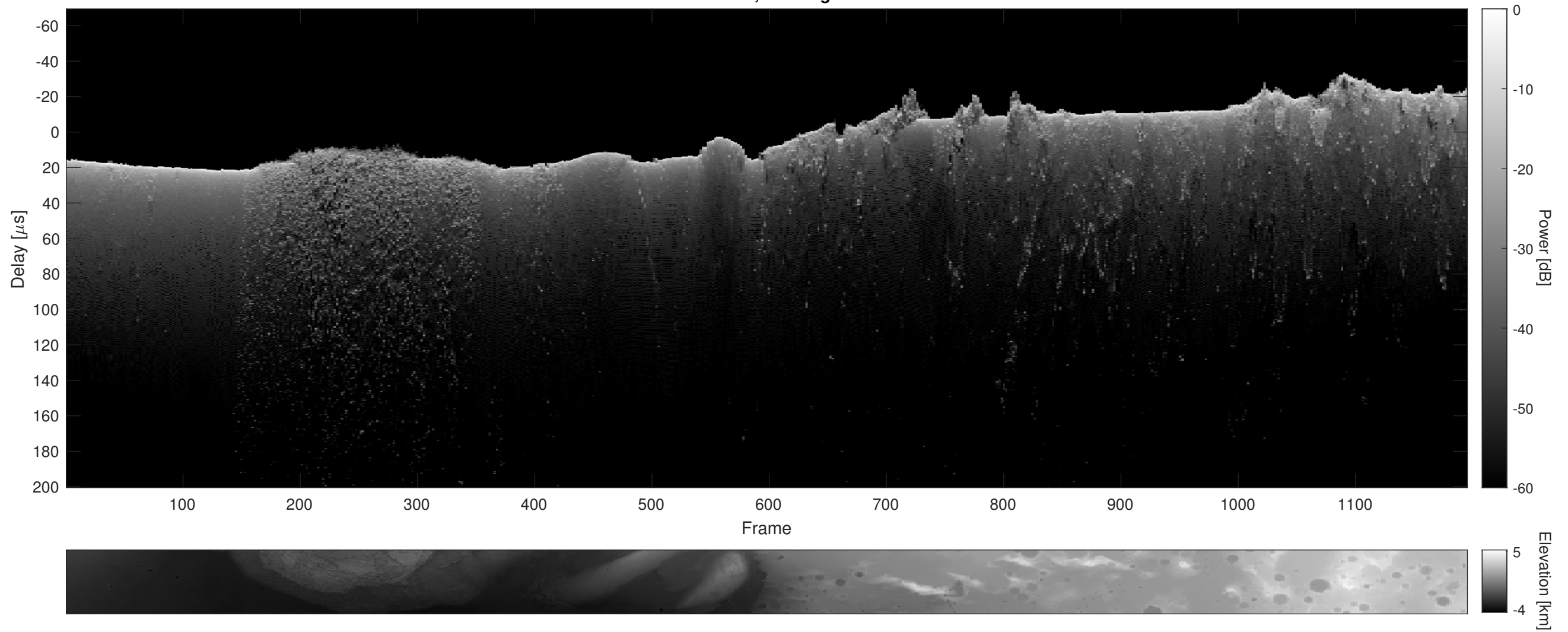
Orbit 7152, Cluttergram
