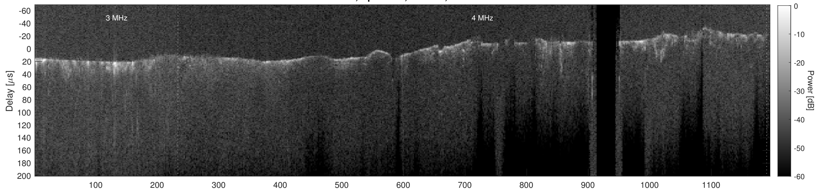
Orbit 7152, Cluttergram
