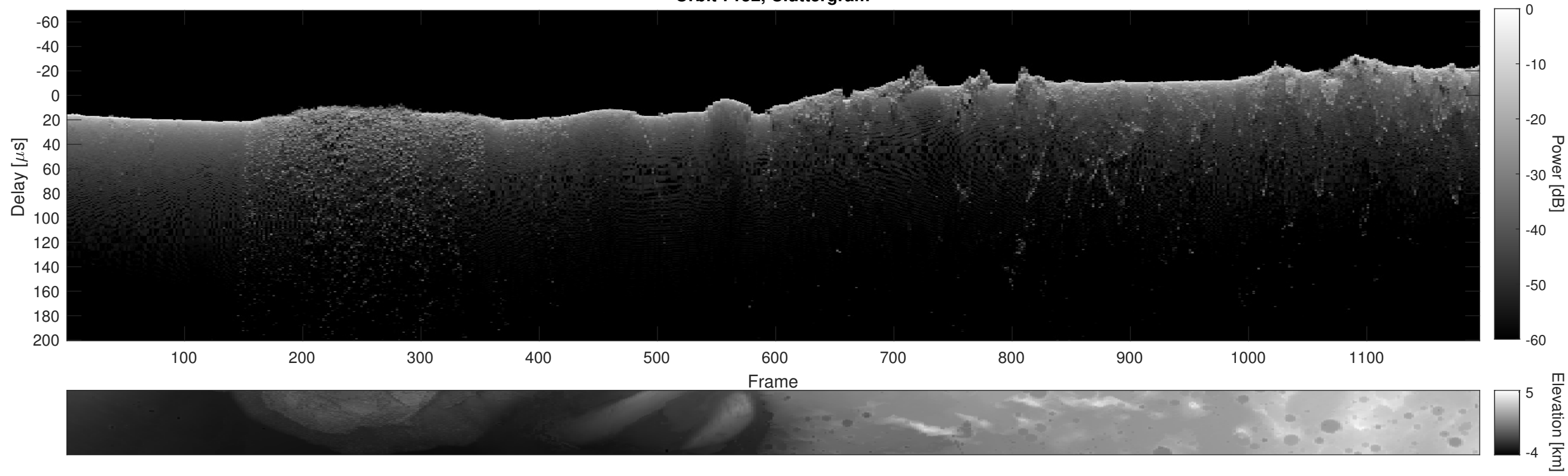
Orbit 7152, Cluttergram
