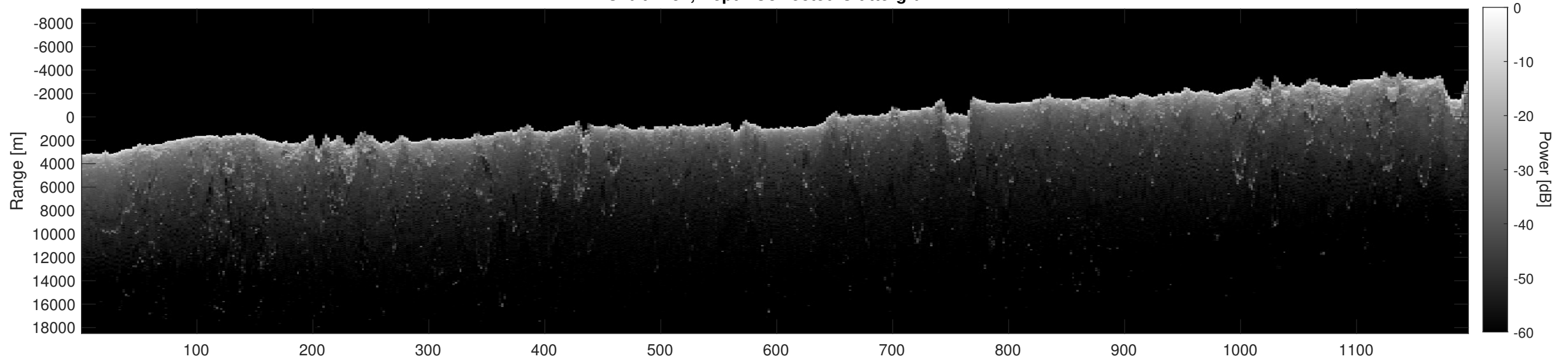
Orbit 7154, Depth-Corrected Cluttergram
