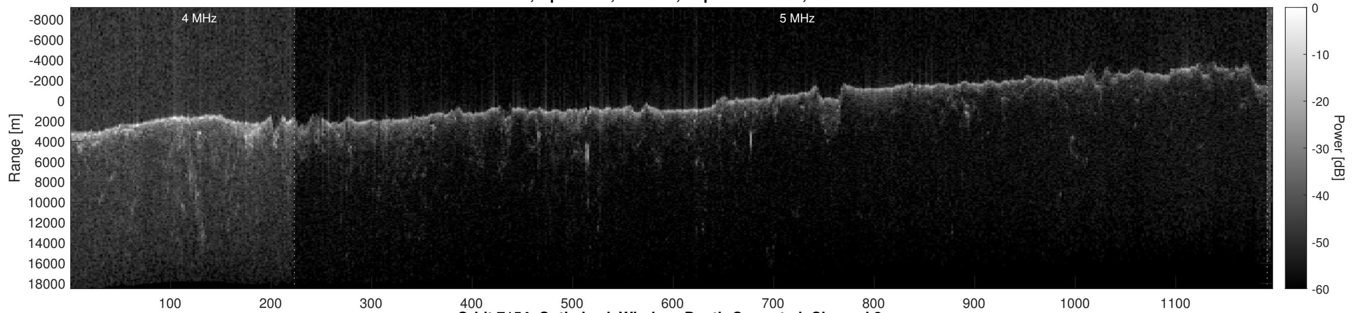
Orbit 7154, Optimized, Window, Depth-Corrected, Channel 2
