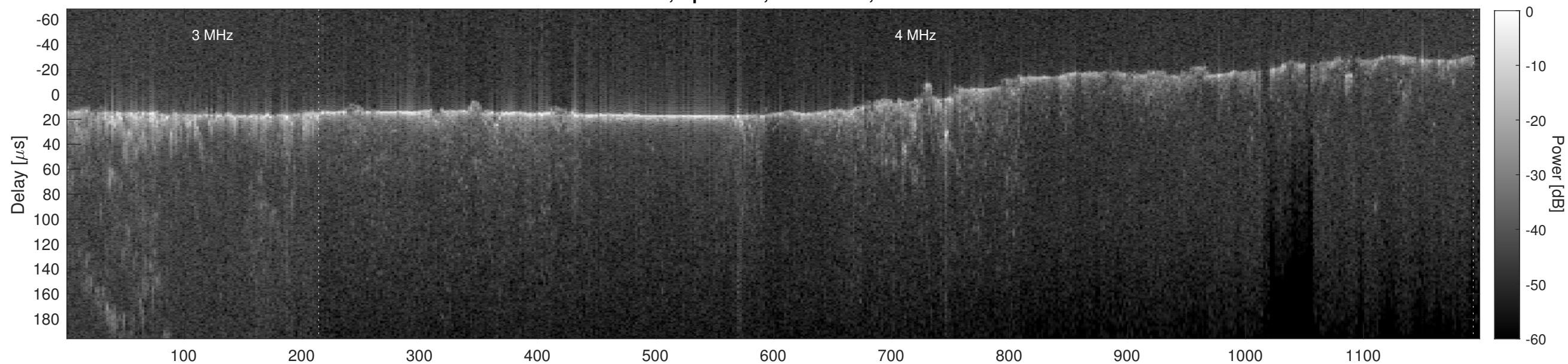
Orbit 7156, Cluttergram
