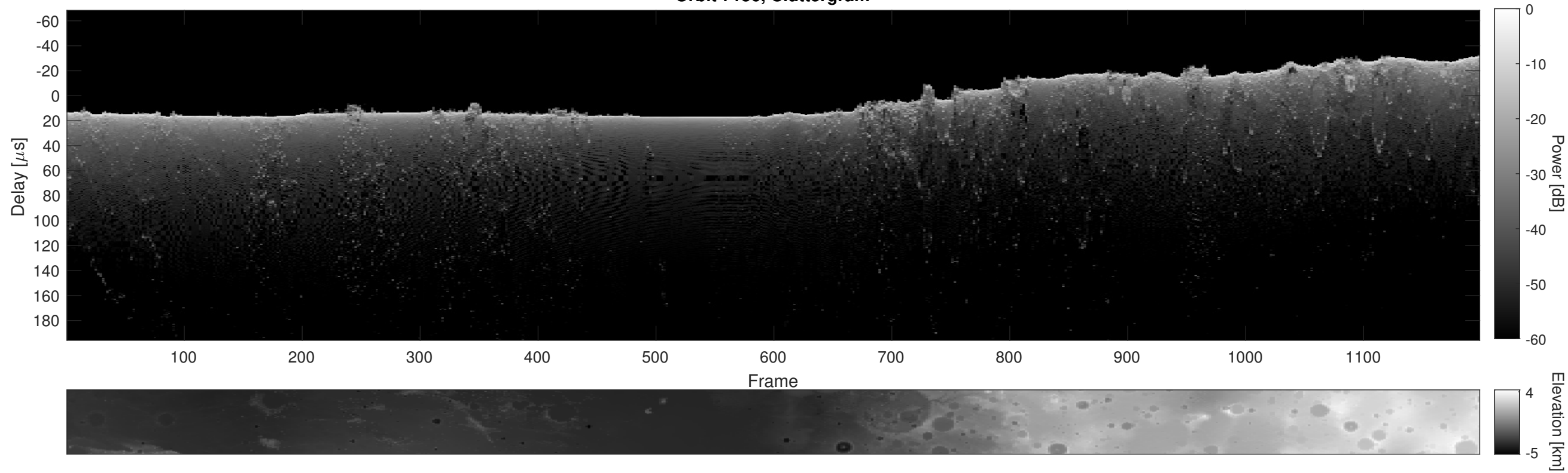
Orbit 7156, Cluttergram
