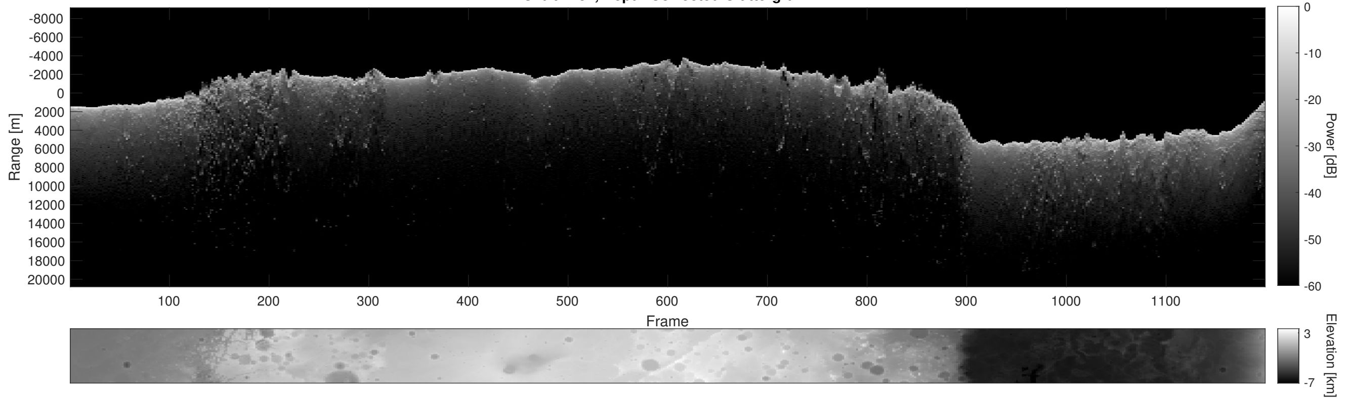
Orbit 7157, Depth-Corrected Cluttergram
