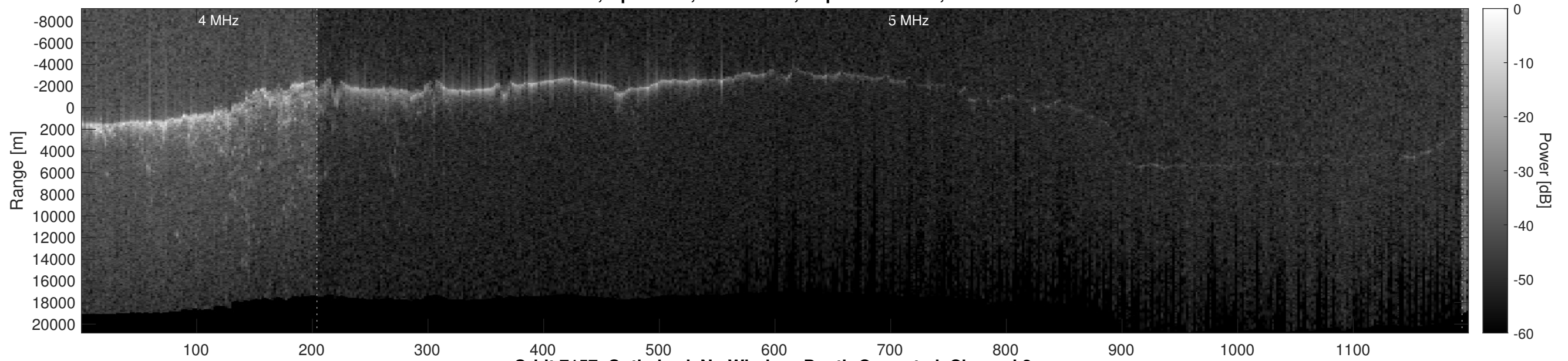
Orbit 7157, Optimized, No Window, Depth-Corrected, Channel 2
