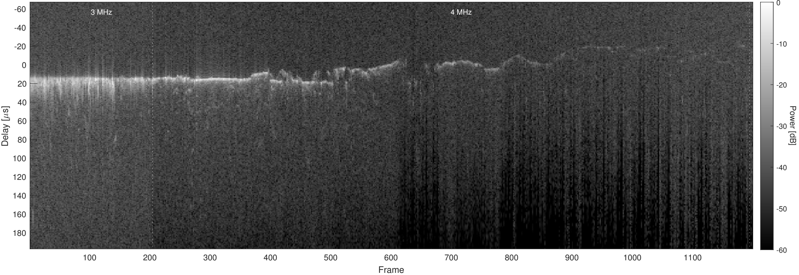
Orbit 7158, Optimized, No Window, Channel 2
