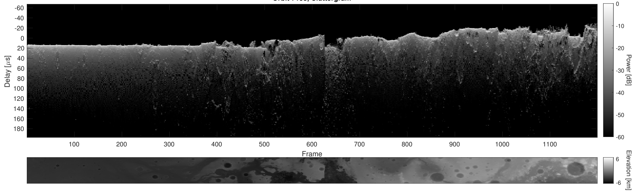
Orbit 7158, Cluttergram
