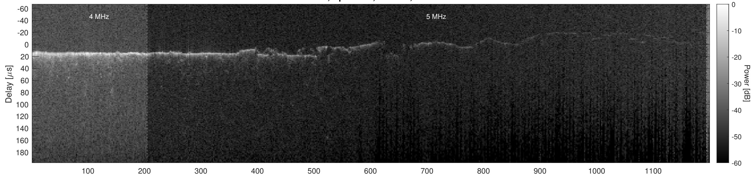
Orbit 7158, Optimized, Window, Channel 2
