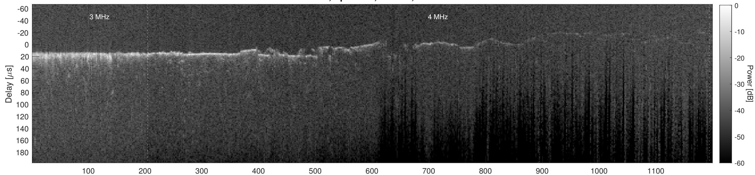
Orbit 7158, Cluttergram
