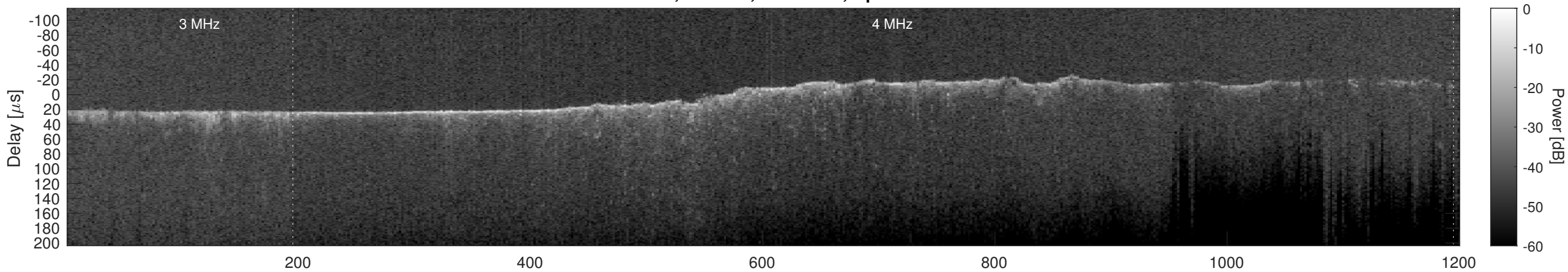
Orbit 7160, Cluttergram
