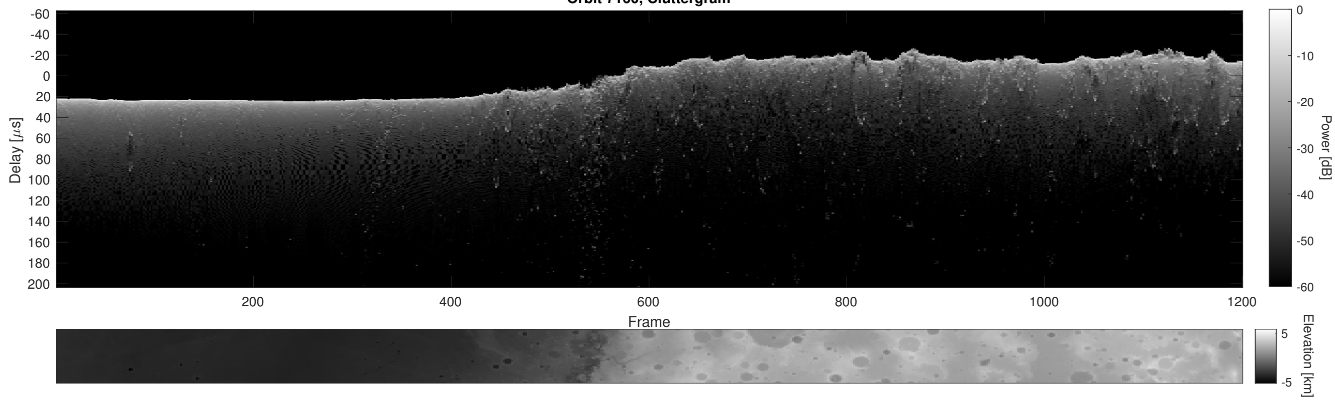
Orbit 7160, Cluttergram
