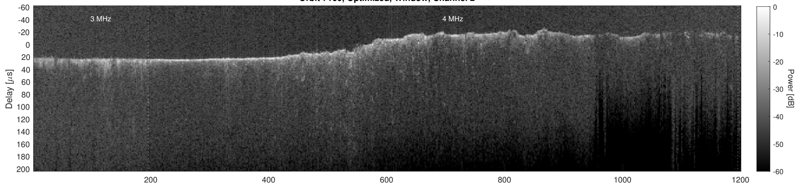
Orbit 7160, Cluttergram
