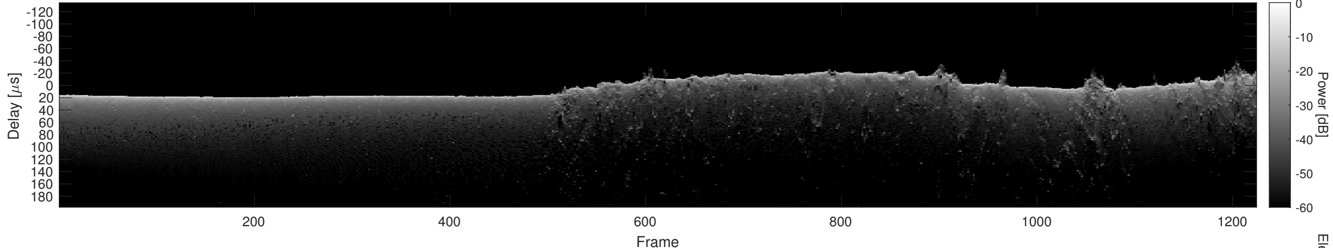
Orbit 7171, Cluttergram
