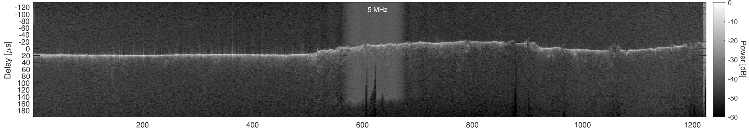
Orbit 7171, Cluttergram
