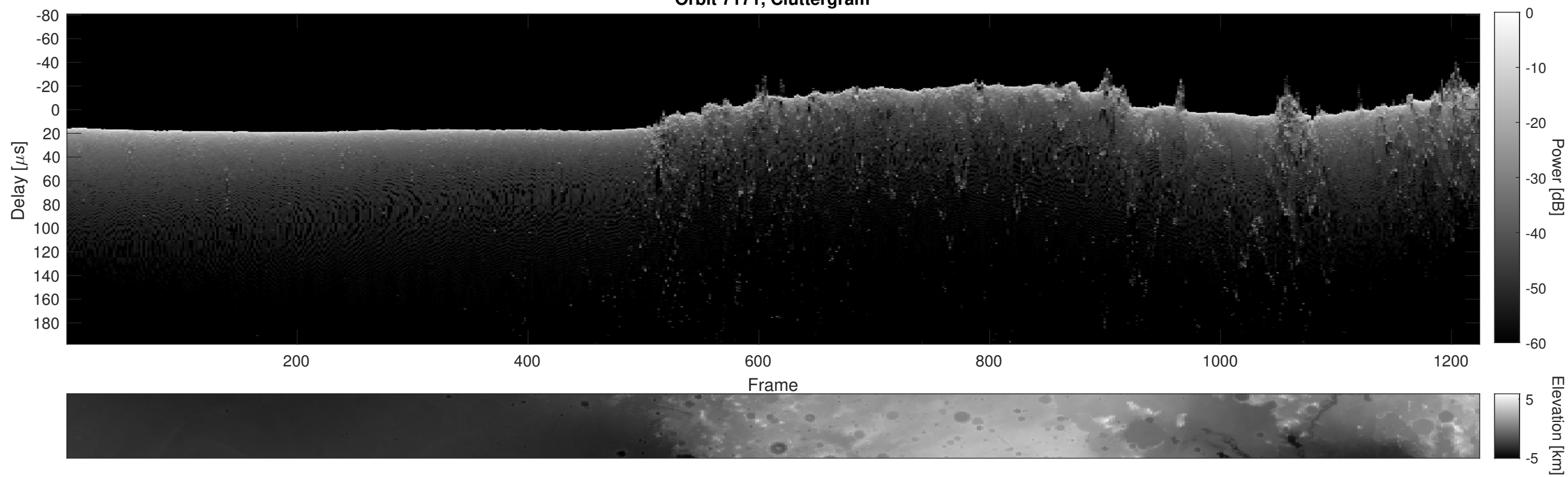
Orbit 7171, Cluttergram
