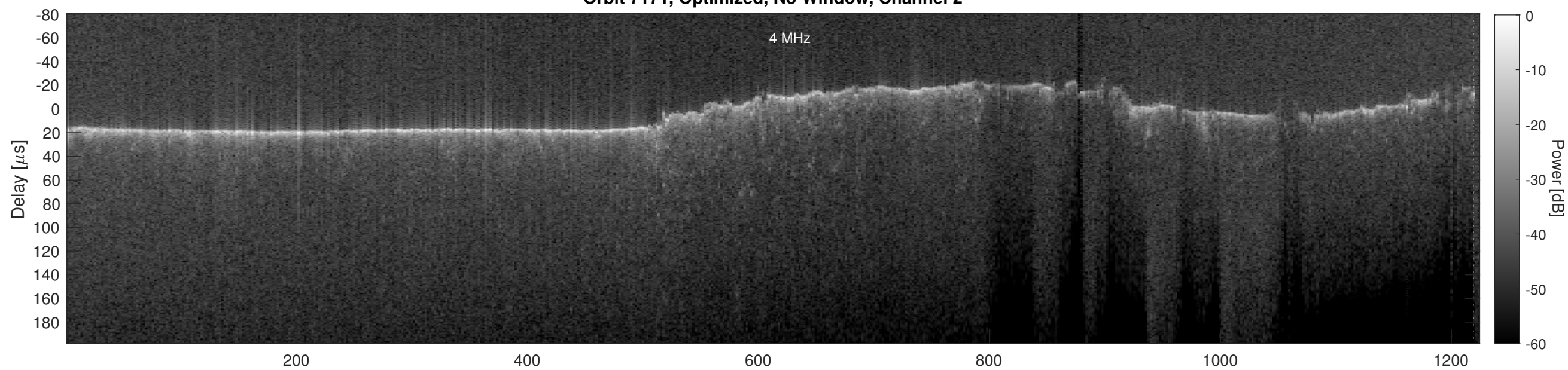
Orbit 7171, Cluttergram
