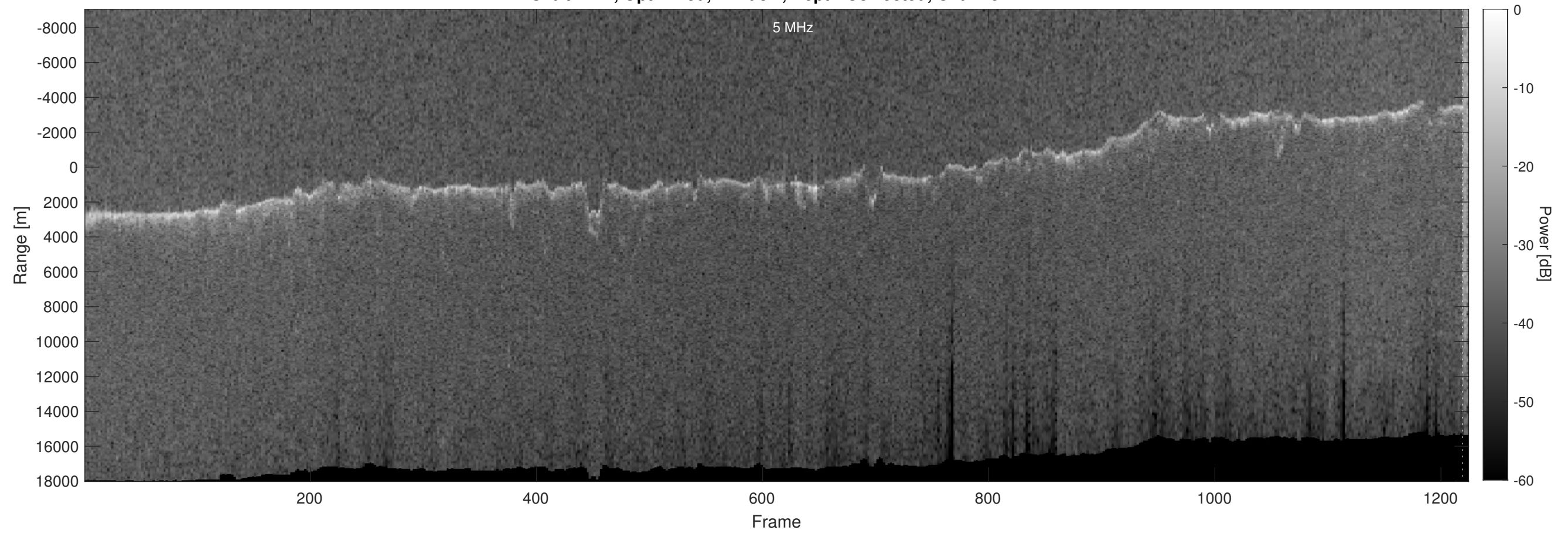
Orbit 7172, Optimized, Window, Depth-Corrected, Channel 2
