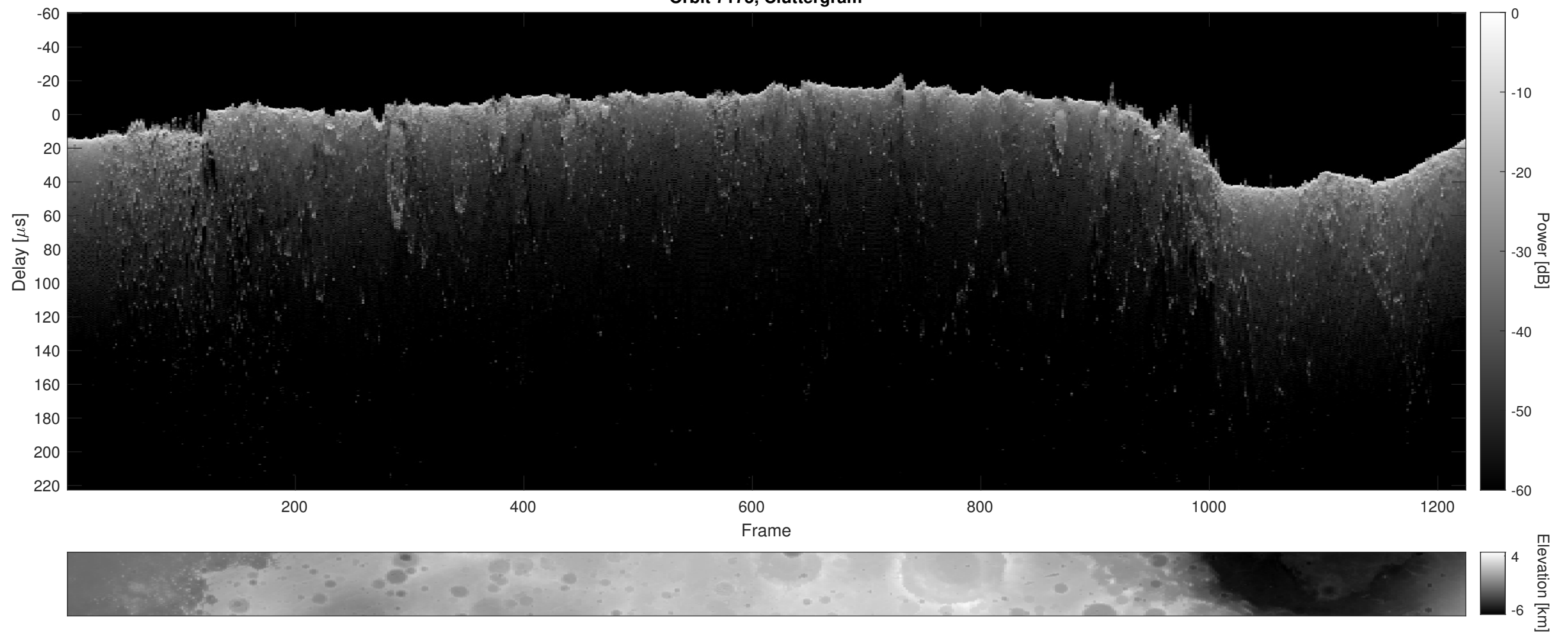
Orbit 7175, Cluttergram
