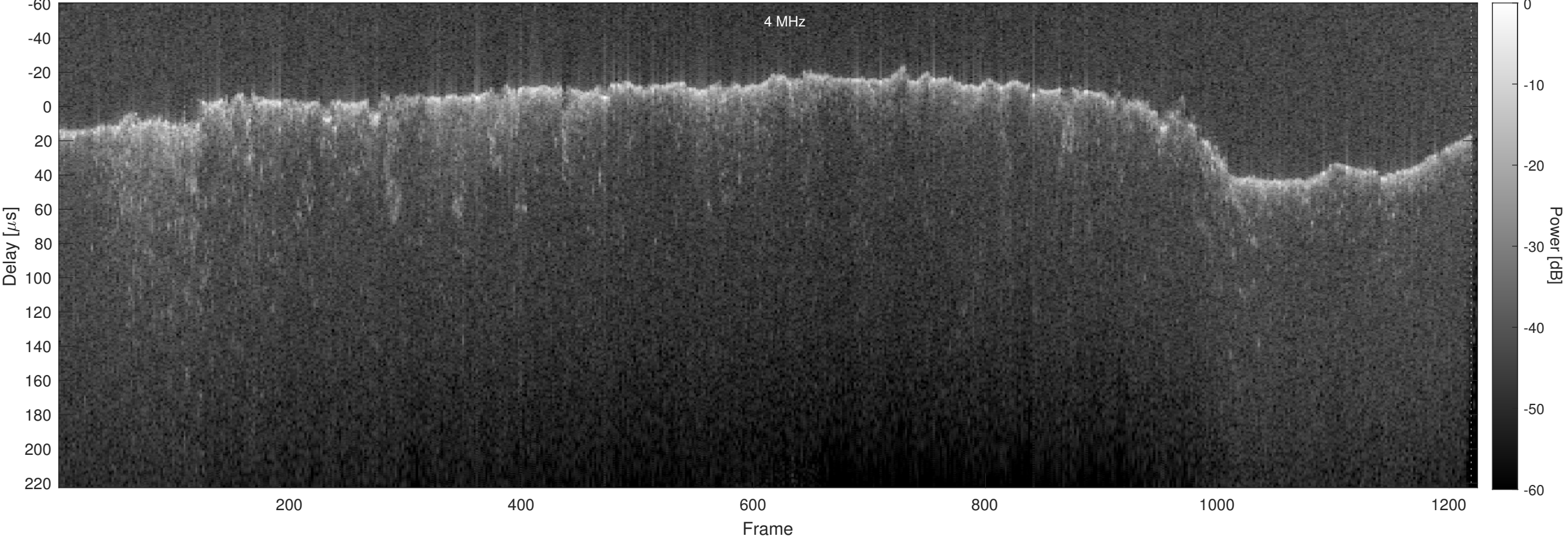
Orbit 7175, Optimized, No Window, Channel 2
