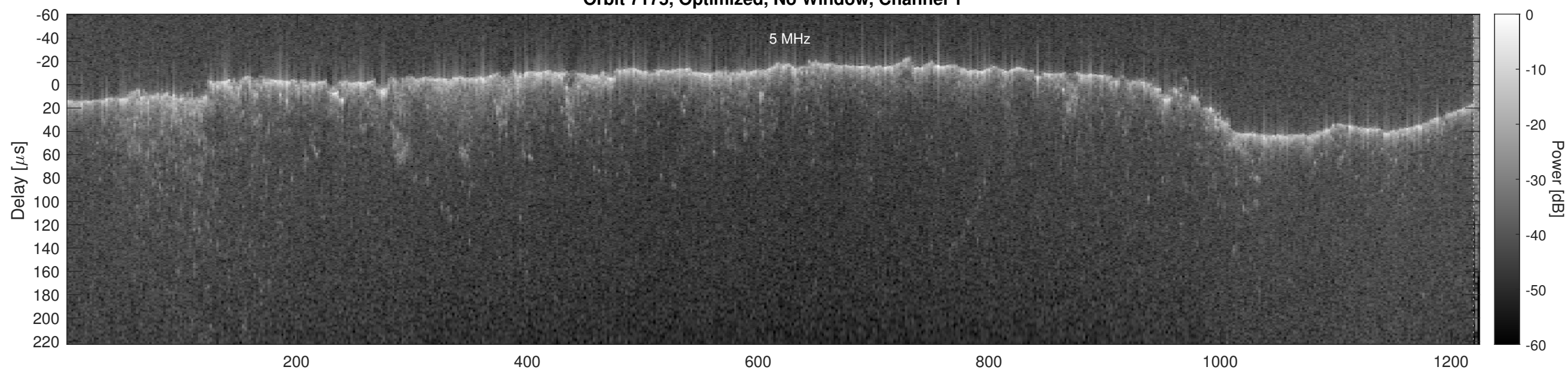
Orbit 7175, Optimized, No Window, Channel 2
