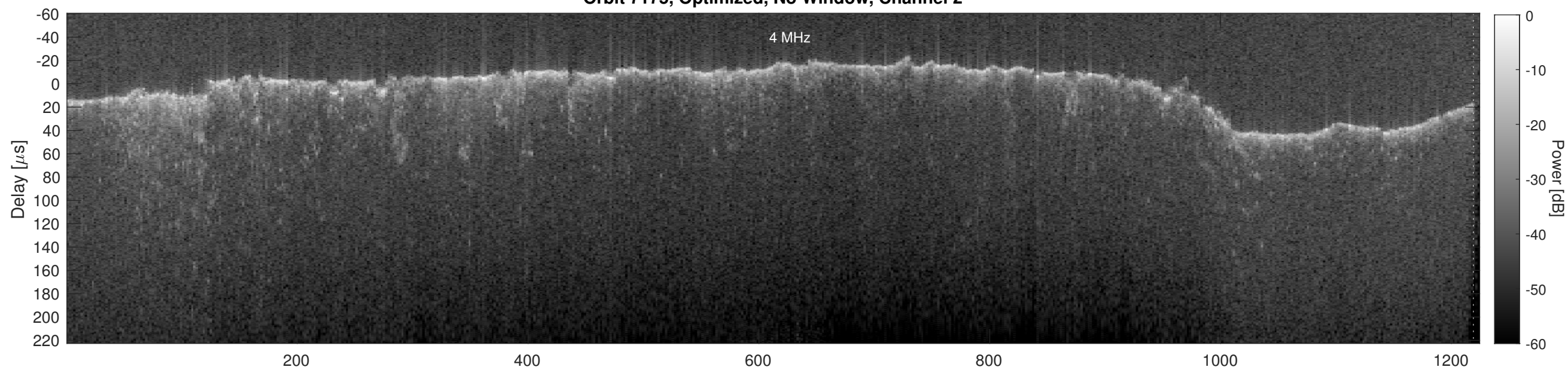
Orbit 7175, Cluttergram
