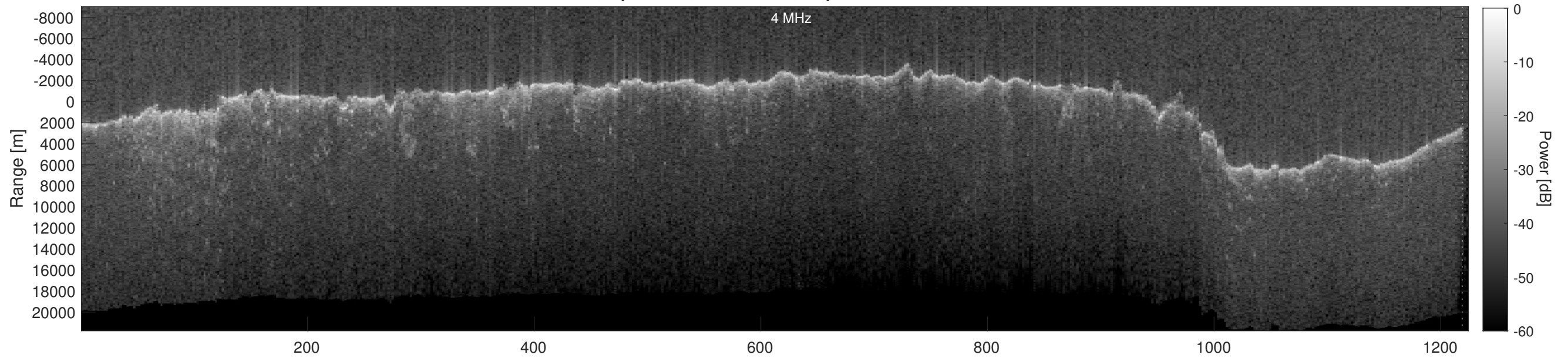
Orbit 7175, Depth-Corrected Cluttergram
