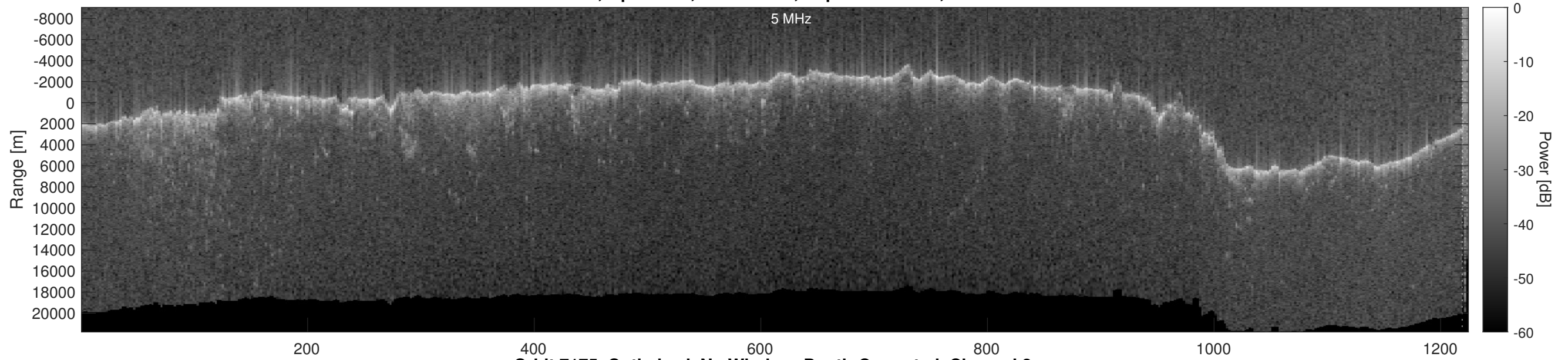
Orbit 7175, Optimized, No Window, Depth-Corrected, Channel 2
