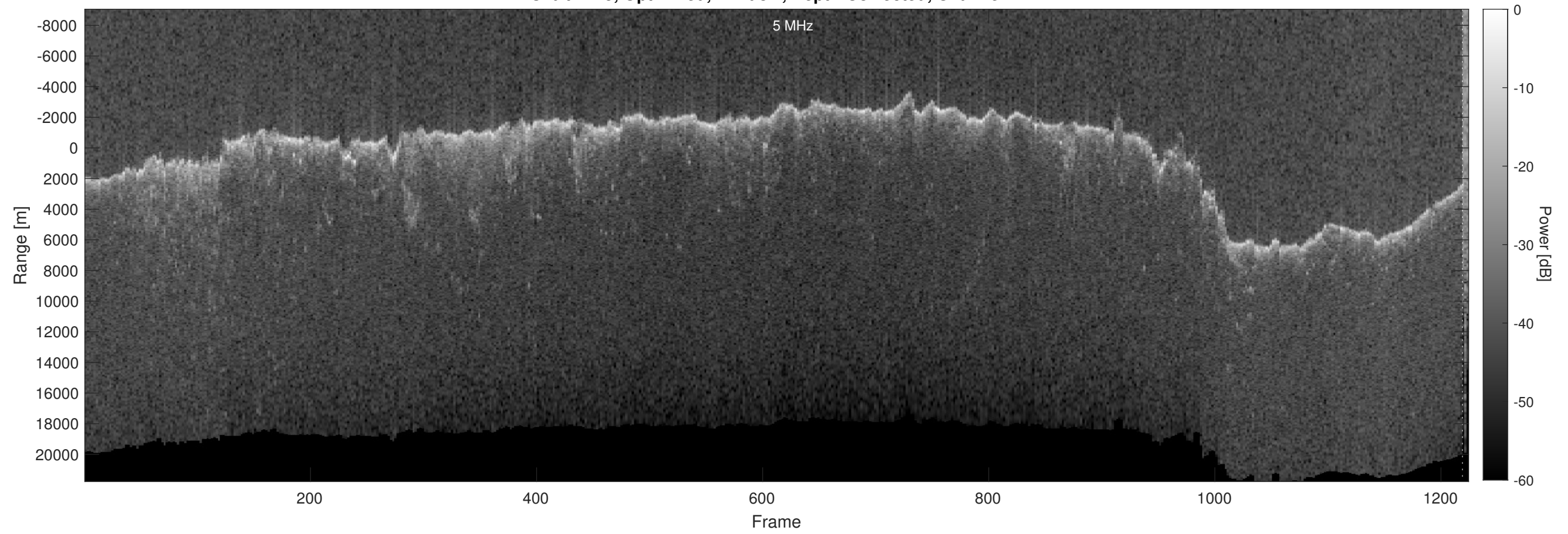
Orbit 7175, Optimized, Window, Depth-Corrected, Channel 2
