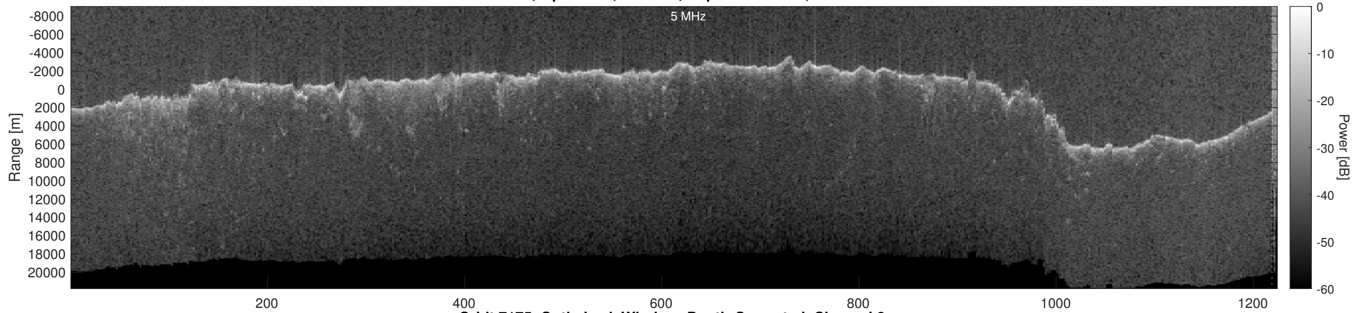
Orbit 7175, Optimized, Window, Depth-Corrected, Channel 2
