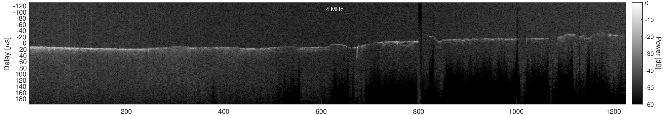
Orbit 7177, Cluttergram
