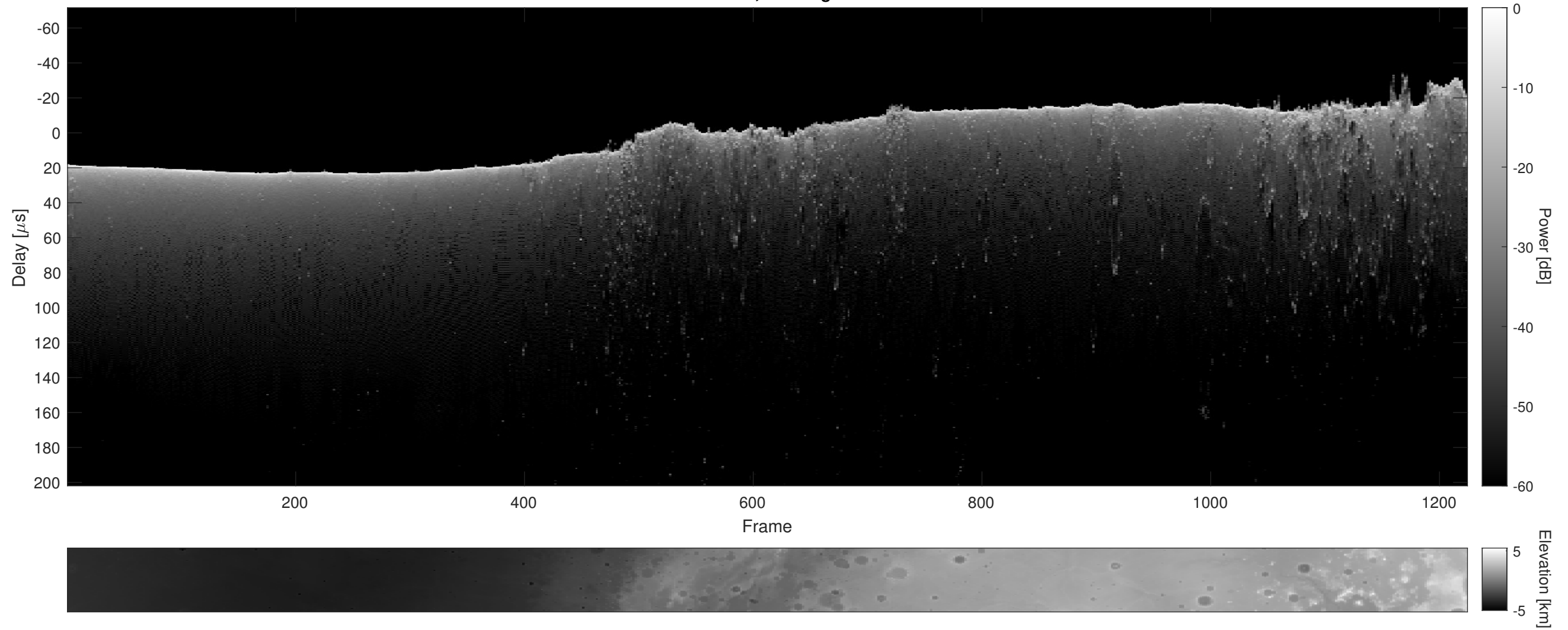
Orbit 7178, Cluttergram
