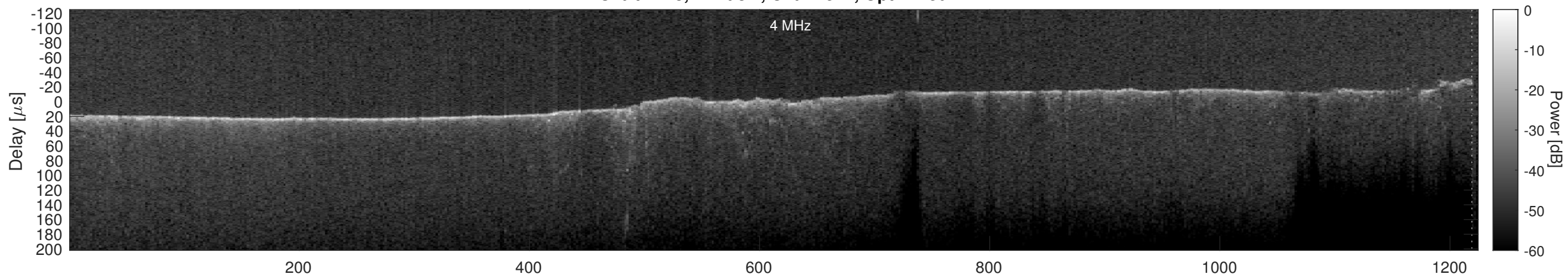
Orbit 7178, Cluttergram
