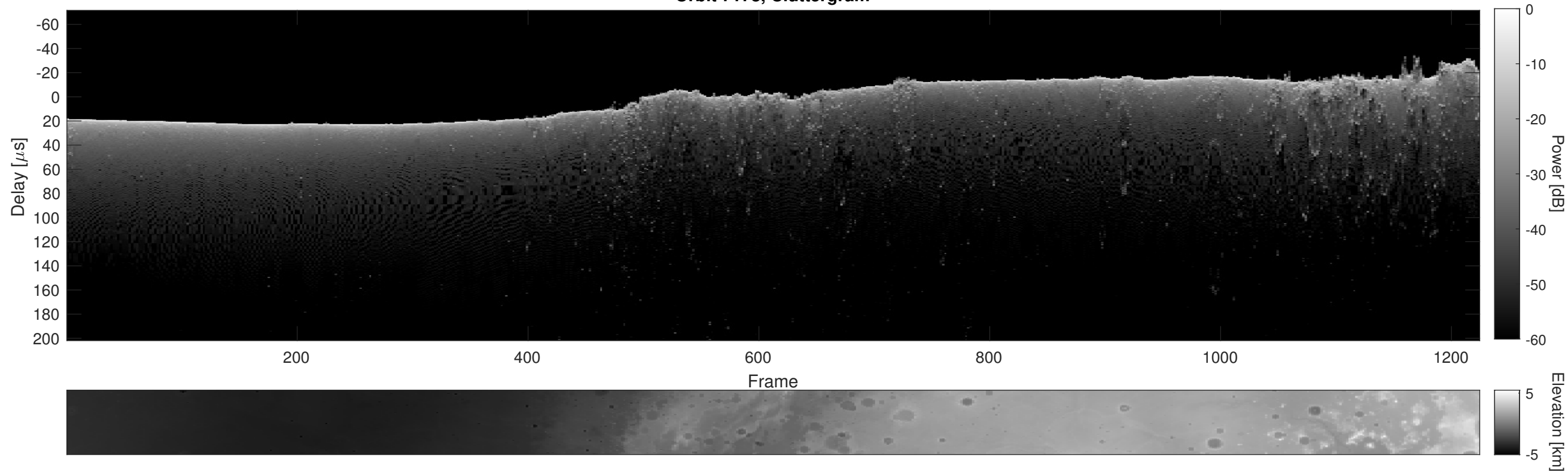
Orbit 7178, Cluttergram
