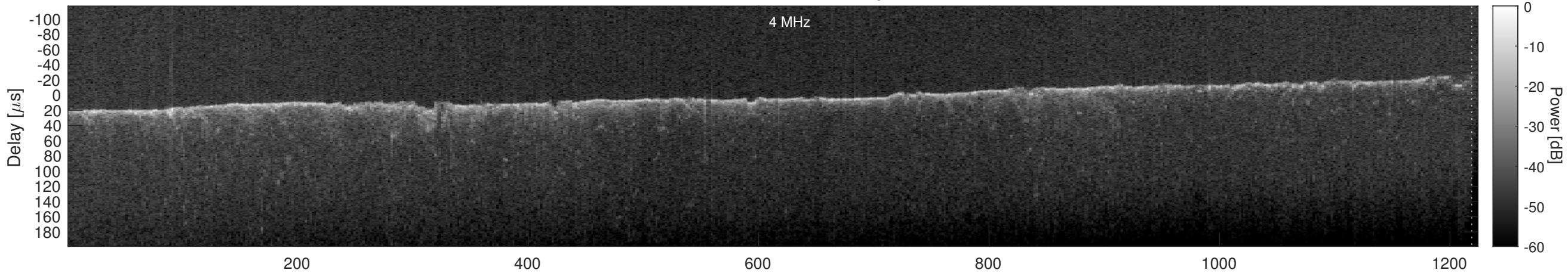
Orbit 7179, Cluttergram
