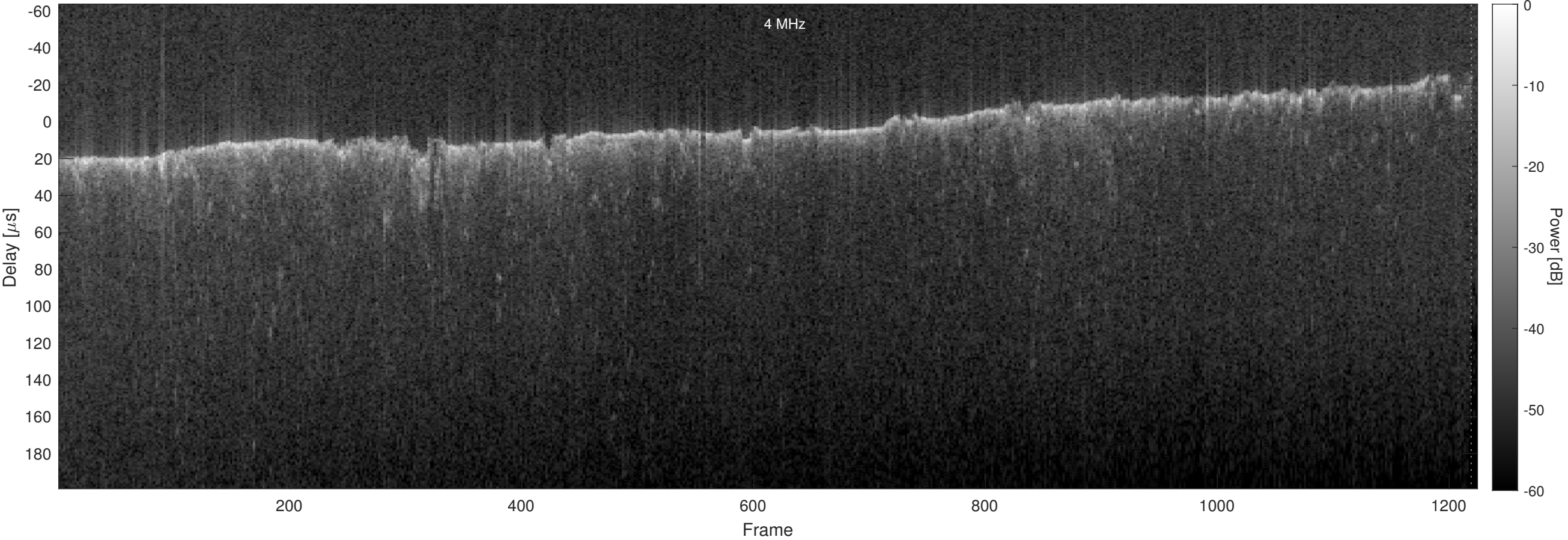
Orbit 7179, Optimized, No Window, Channel 2
