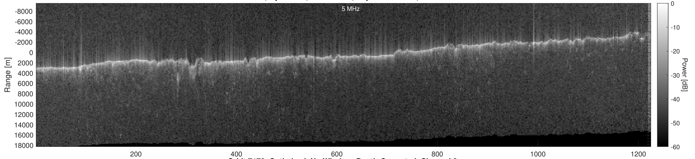
Orbit 7179, Optimized, No Window, Depth-Corrected, Channel 2
