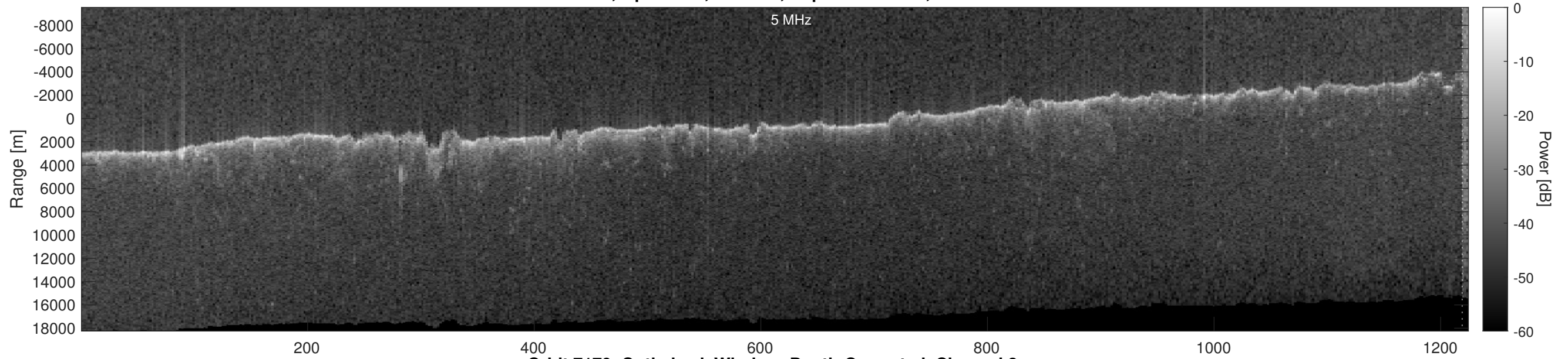
Orbit 7179, Optimized, Window, Depth-Corrected, Channel 2
